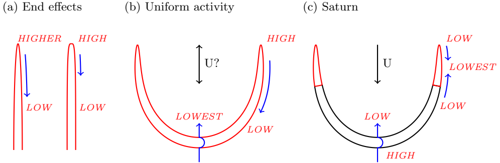
Figure 8: Qualitative schematic: understanding end shape and azimuthal effects. Red text indicates the relative concentration of solute in each figure, with slip flow (blue) moving from higher to lower concentrations, assuming constant, negative mobility. a) The shape of the filaments affects the geometric confinement at the ends, resulting in different strength of slip flows. b) A uniformly active prolate spheroid. For our parameter choices, azimuthal flows work in opposition to axial flows and hence the swimming direction is sensitive to which effect is stronger, which in turn depends on geometry and end shape. c) In a capped filament azimuthal flows and axial flows work together, however there is an opposing end-effect flow (as with the Janus prolate spheroid) that slows the swimmer.
