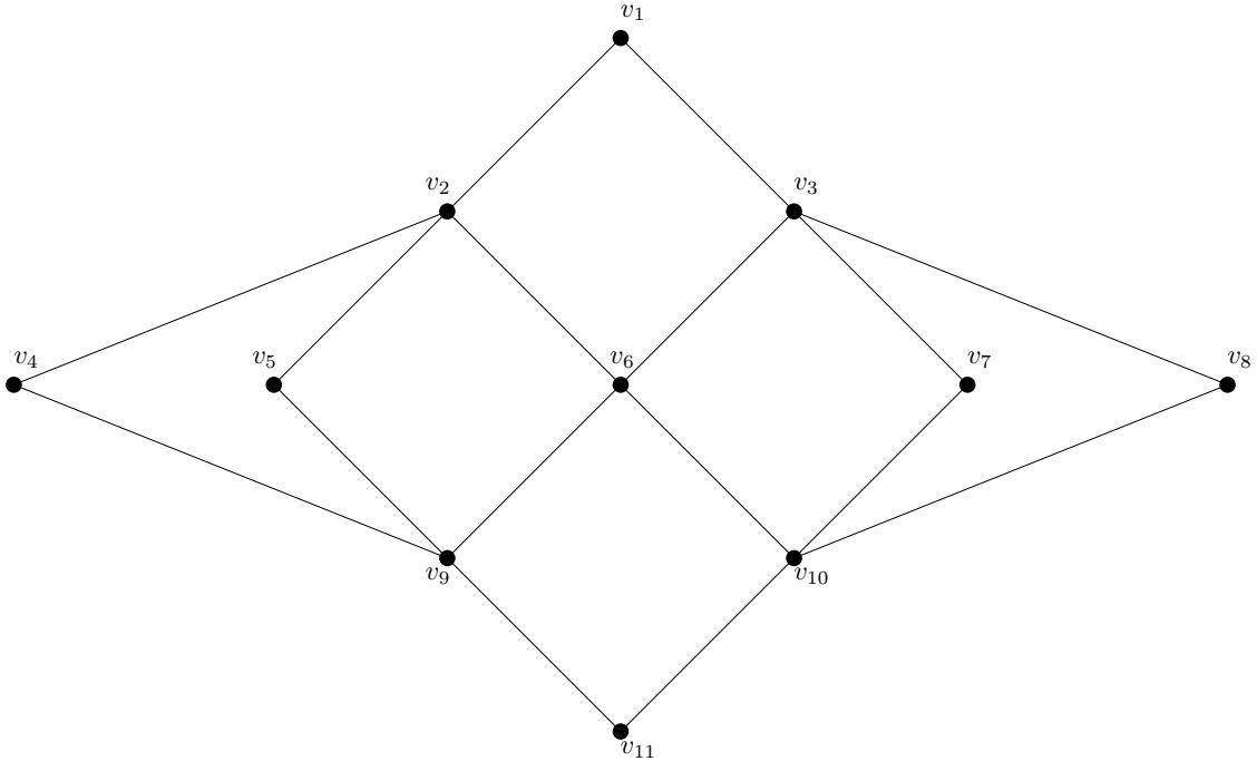
FIGURE 2. The Hasse diagram of the poset H
