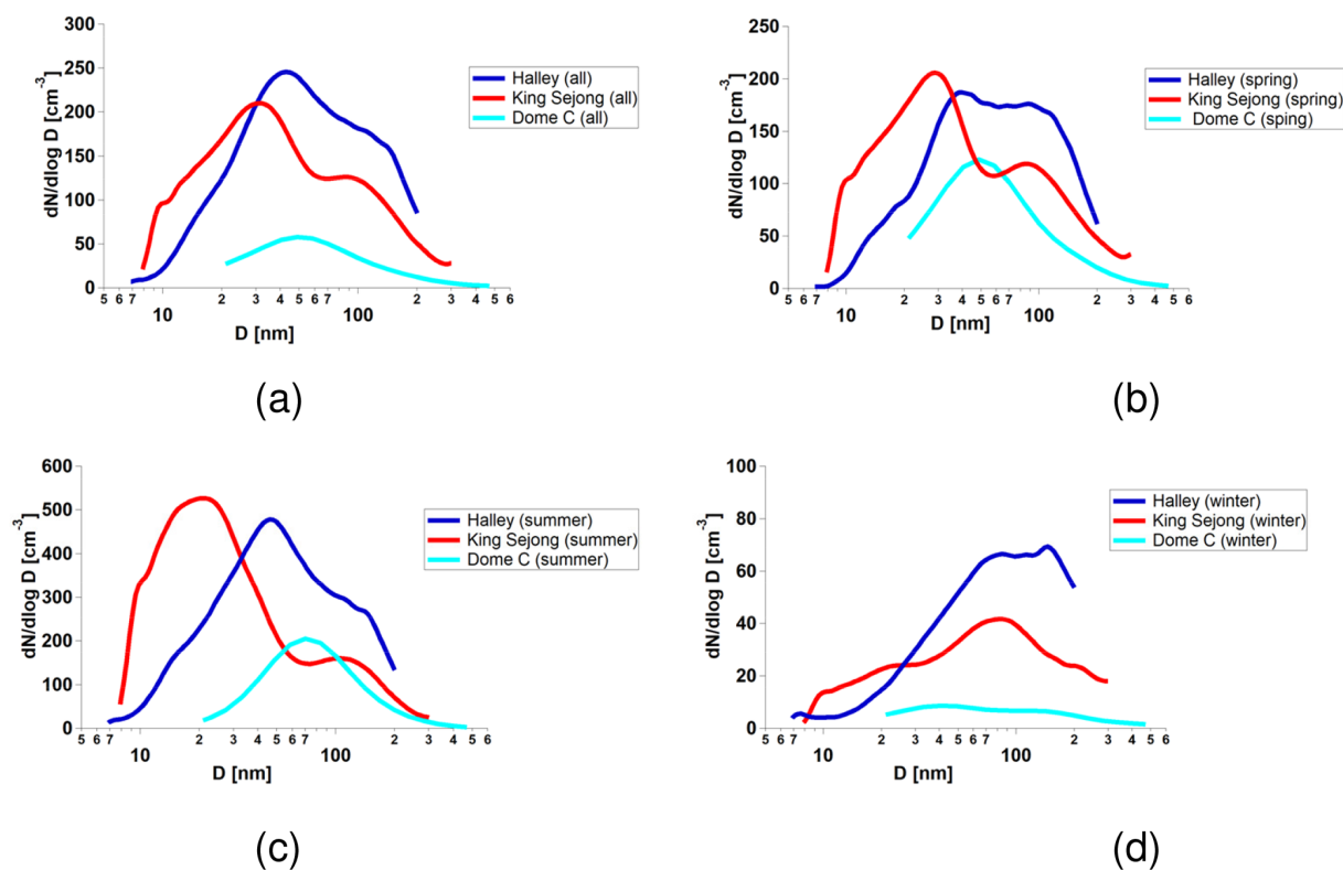
Figure 6. Average size-resolved particle size distributions simultaneously measured during the year 2015 at Halley, Dome C and King Sejong stations for (a) May–December (8 months), (b) spring (September, October and November; 3 months), (c) summer (December; 1 month) and (d) winter (June, July and August; 3 months). D : diameter.
