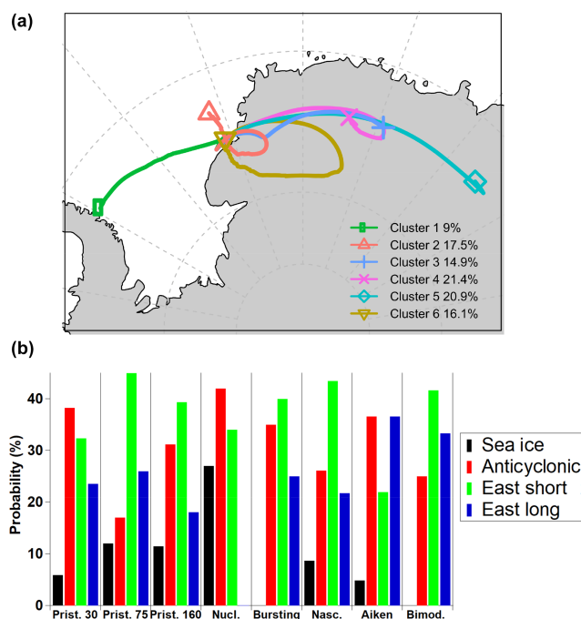
Figure 4. (a) Air mass analysis of air mass back trajectories arriving at Halley during the year 2015 (hourly resolution) and (b) relative contribution for each aerosol category. Groups in (b) are sea ice (1), anticyclonic (2, 6), east short (3, 4) and east long (5).
