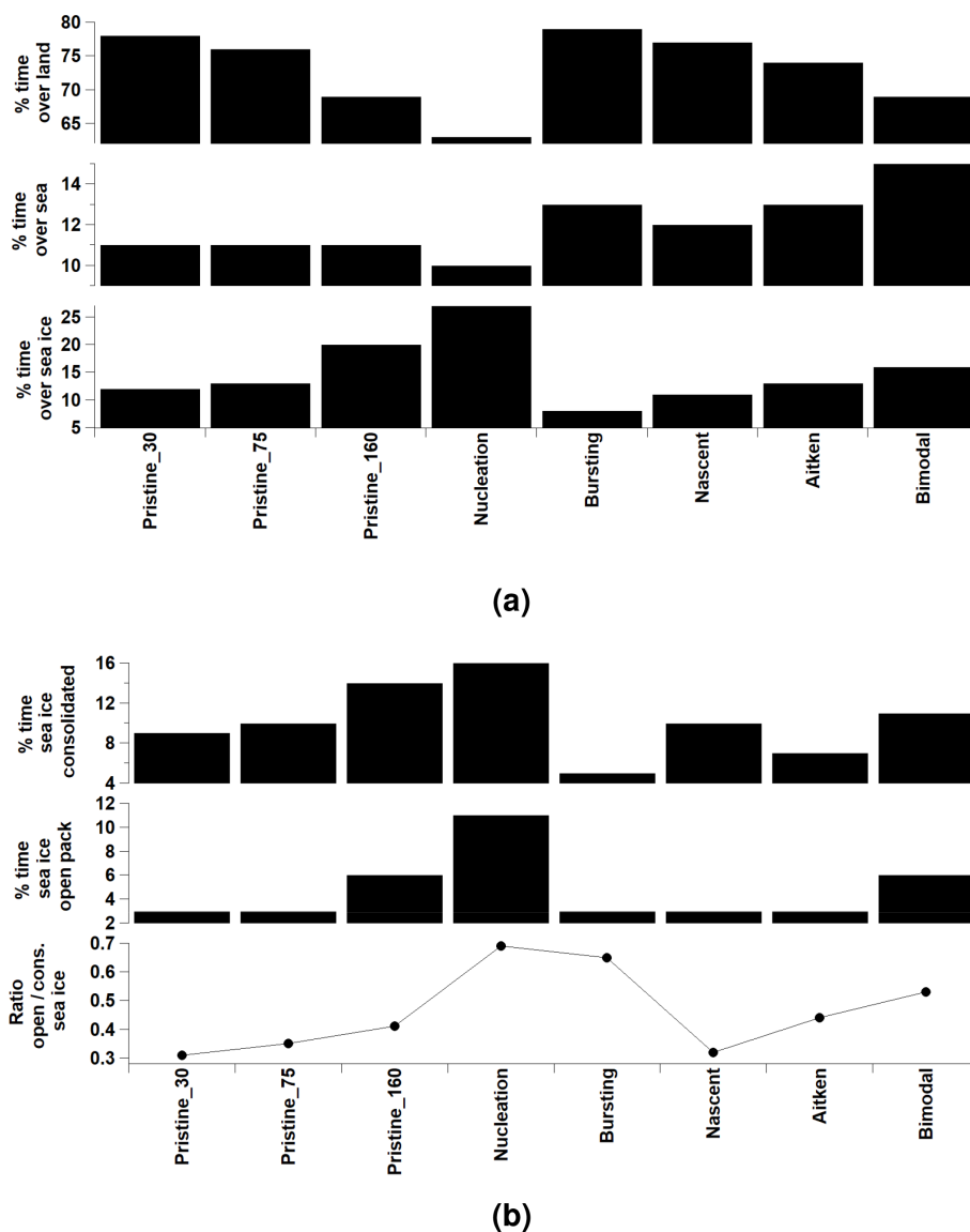
Figure 5. (a) Percentages of air masses over land, sea and sea ice for the eight k -mean aerosol categories and (b) percentages of consolidated and open-pack sea ice and the ratio of open-pack/consolidated sea ice.
