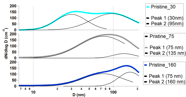
Figure 3. Peak fitting of the three pristine k -mean aerosol categories. D : diameter.
