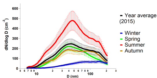
Figure 1. Seasonal mean aerosol size distribution measured by the SMPS at Halley VI over the year 2015. The error bars represent the standard deviation of the measurements from the mean value. D : diameter.
