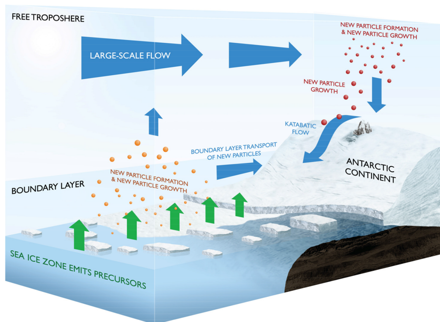
Figure 8. Schematic illustrations of the ultrafine new particle formation (NPF) and new particle growth (NPG) aerosols in Antarctica.
