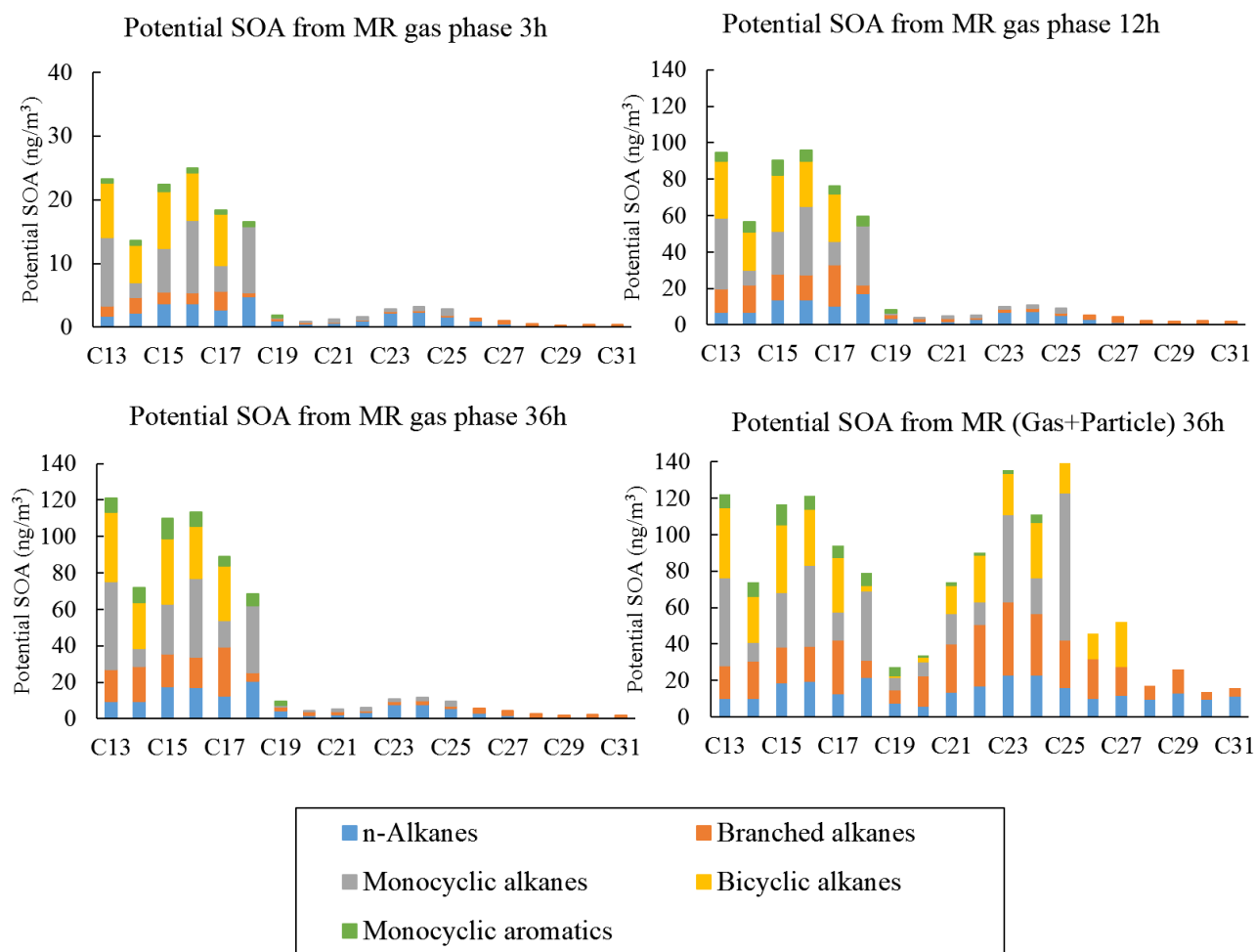
Figure 5. The potential SOA formation in the 3h, 12h, 36h calculated from MR I/SVOCs.
