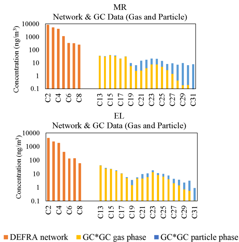
Figure 1. Average concentrations of n-alkanes from the DEFRA network ( C_2 - C_8 ) and GC \times GC-MS ( C_{13} - C_{31} in the gas phase and particle phase) at MR (top panel) from March to April 2017 and at EL (bottom panel) from February to March 2017.
