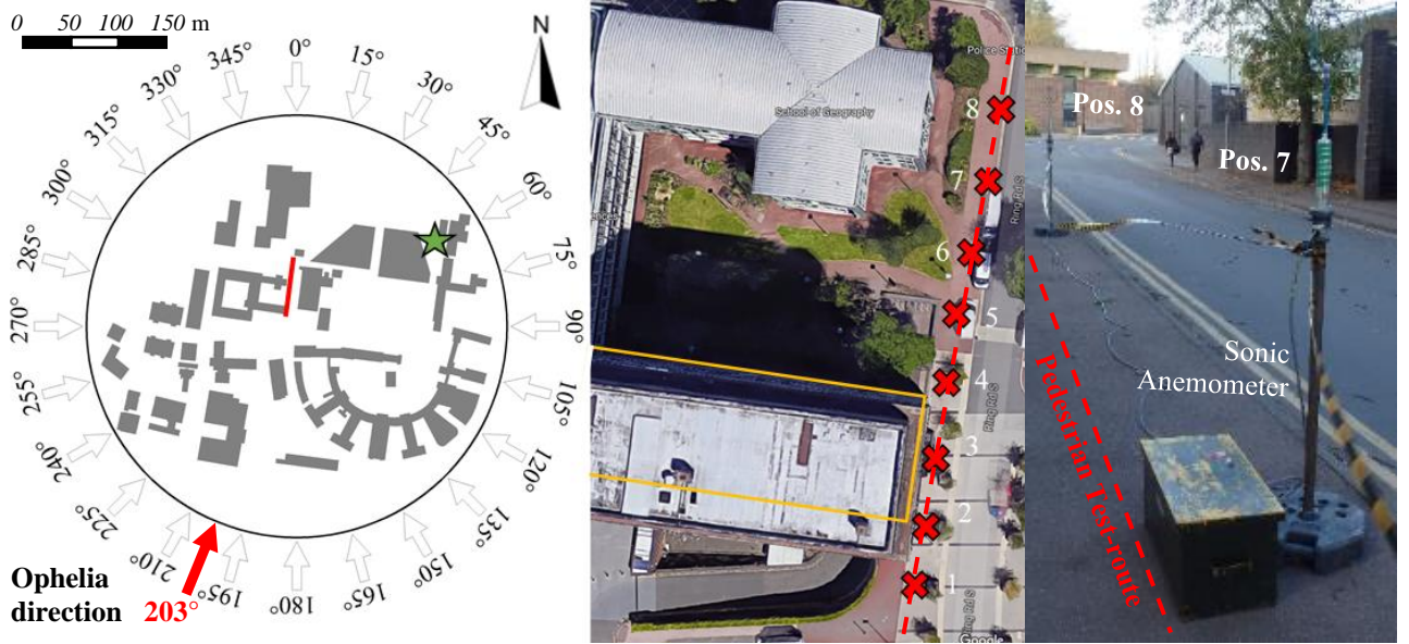
Figure 3. Full Scale Experiment. (Left) Map of UoB campus, with footpath alignment at the base of the BB and reference point position on top of the MT, with cardinal directions; (centre) Aerial view of footpath and position of 8 sonic anemometers (Map data ©2019 Google); (Right) view of sonic anemometers as installed during the measurement campaign.
