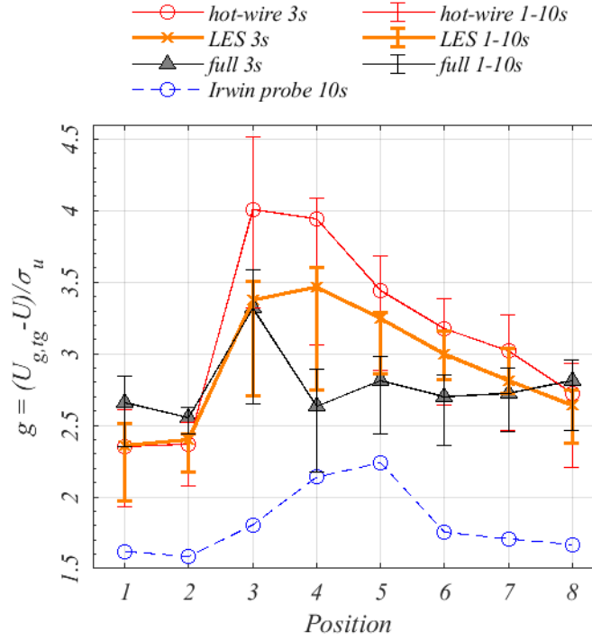
Figure 20. Peak factor g , as predicted with gust wind speeds U_{g,tg} for Irwin probes, hot-wire anemometry, and LES, compared to full-scale. The error bars show the gust duration effect on the peak value, with upper and lower bars showing respectively the 1 s and 10 s gusts.
