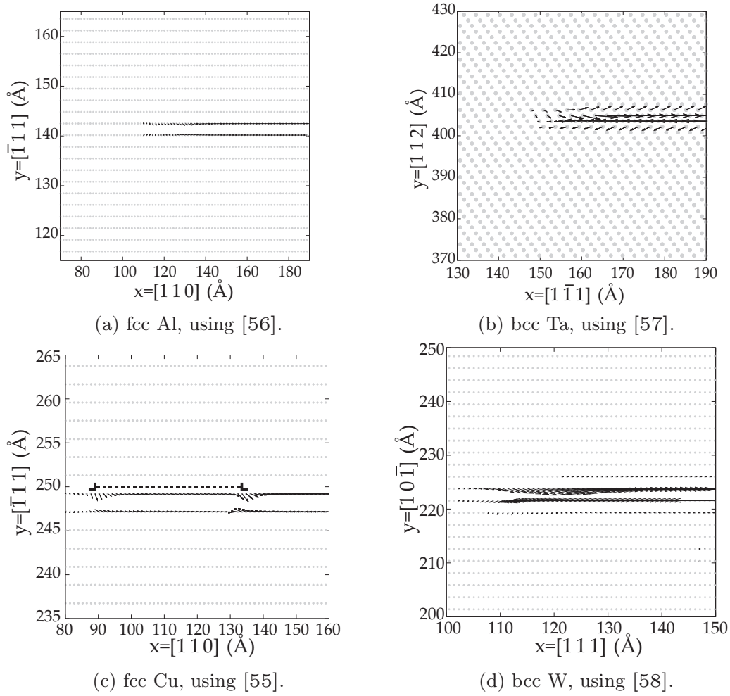
FIG. 3. Kanzaki core fields corresponding to the affine maps in Fig. 2. The scale for the forces is 1 \text{ Å} \equiv 1 \text{ eV/Å} .
