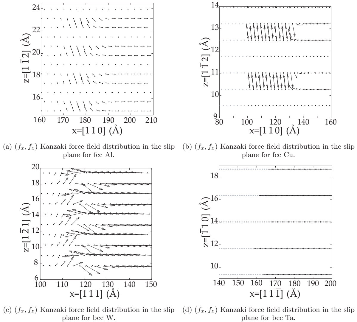
FIG. 7. Antiplanar Kanzaki field components. The scale is 1 \text{ Å} \equiv 1 \text{ eV/Å} , except for Fig. 7(d), where the scale is 1 \text{ Å} \equiv 2 \text{ eV/Å} .
