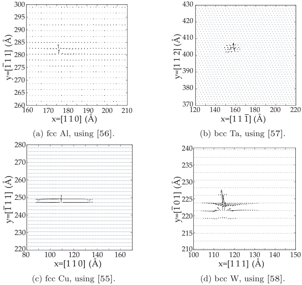
FIG. 5. Core Kanzaki forces for the reference materials. Scale of 1 \text{ \AA} \equiv 1 \text{ eV/\AA} .
