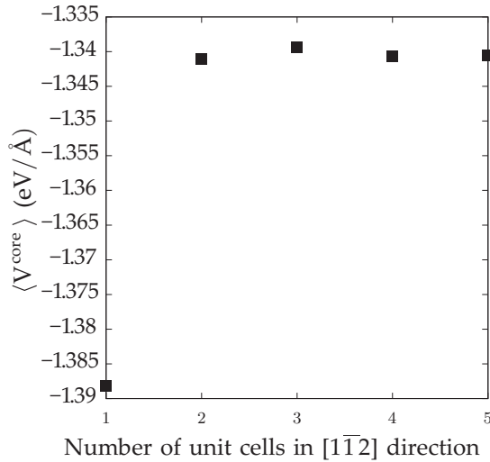
FIG. 8. Average core energy for fcc Al.
