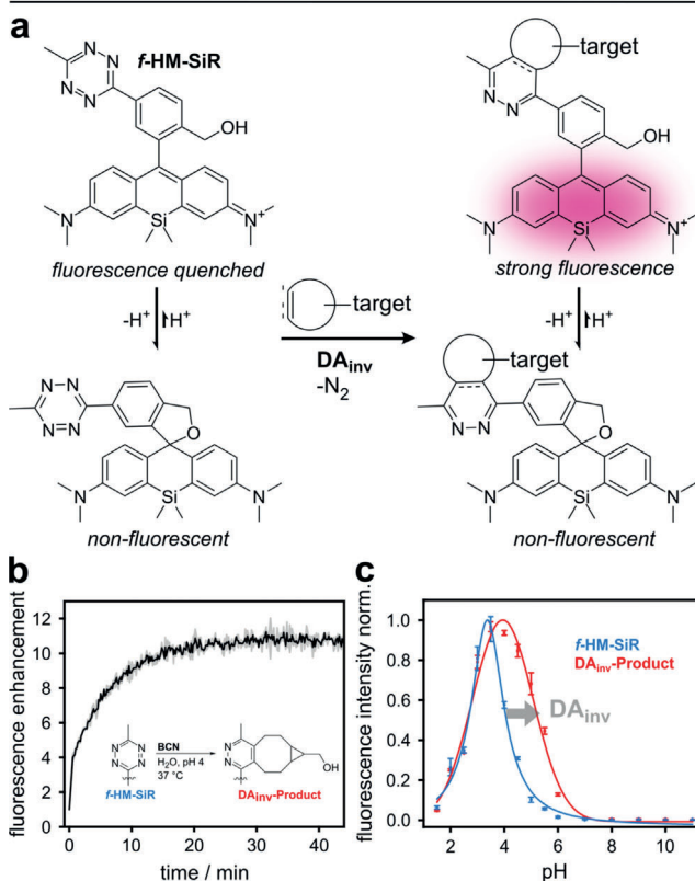
Figure 1. f-HM-SiR , a fluorogenic and spontaneously blinking fluorophore for bioorthogonal \text{DA}_{\text{inv}} . a) Spiro-cyclization equilibrium of spontaneously blinking and fluorogenic f-HM-SiR and its Diels–Alder cycloadduct ( DA inv -Product ). b) Fluorescence enhancement of f-HM-SiR upon conversion in \text{DA}_{\text{inv}} at pH 4 in aqueous buffer. c) pH-dependent fluorescence of f-HM-SiR (blue) and DA inv -Product (red).
