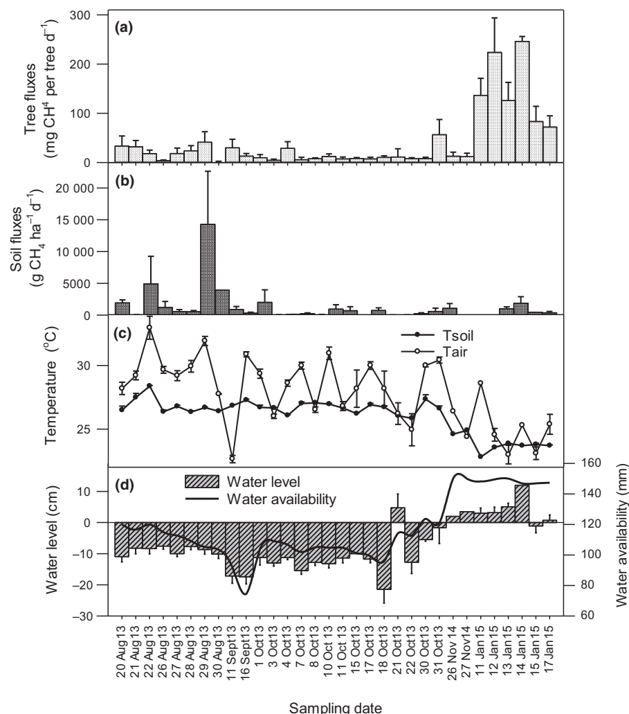
Fig. 4 Temporal variation in (a) \text{CH}_4 emissions from trees across the range of tree species and locations measured in a given day, (b) \text{CH}_4 emissions from soil measured adjacent to the trees measured on the same day, (c) soil and air temperature, and (d) water level and water availability. The figure combines all individual measurement dates at the different sites, as the sampling followed a block structure (Fig. 1). Data from each day include both vegetation types and the full range of species. Means \pm SE are shown.
