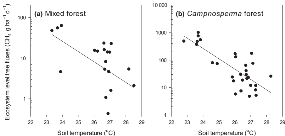
Fig. 7 Relationships between estimated ecosystem-level CH 4 emissions from trees and soil temperature at (a) the mixed and (b) the Campnosperma forest sites. Significant linear regression models are plotted; the models are reported in Table 3.
