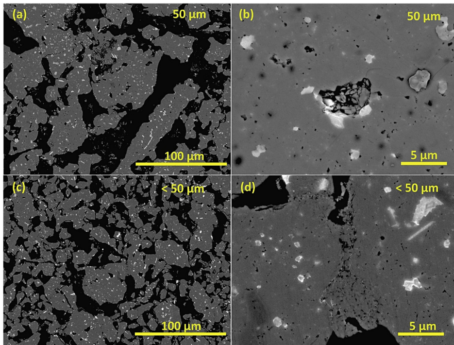
Fig. 10. BSE SEM micrographs of SPS reprocessed finer fractions 50 and <50 \mu\text{m} at 750 ^{\circ}\text{C} .
