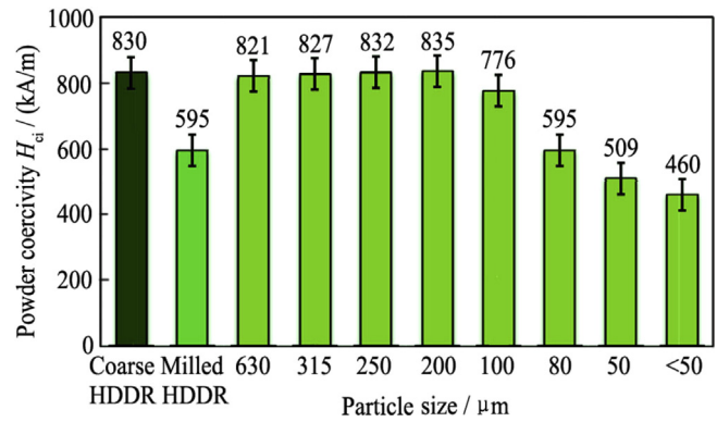
Fig. 6. Coercivity variation with the powder particle size after burr milling.
