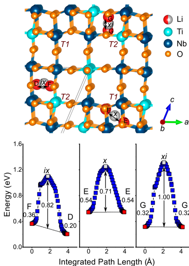
Figure 9. Cross-block Li diffusion pathways and corresponding activation energies in eV. Li minima ( \text{Li}_\text{D} – \text{Li}_\text{G} ) and transition states (configurations ix – xi ) are shown in red and gray, respectively. The energies of the local minima and kinetically-resolved activation energies (eq 1 in the Supporting Information) relative to configuration C are displayed on the conduction barrier plots (blue). An interpolation of the energy between the initial and final minima for each Li hop is shown.
