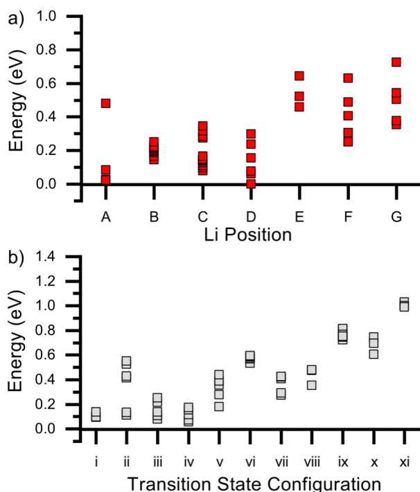
Figure 10. Energies of (a) local Li minima and (b) kinetically-resolved activation barriers in the disordered \text{TiNb}_2\text{O}_7 supercell. Li sites \text{Li}_\text{A} – \text{Li}_\text{G} correspond to the Li positions observed in the ordered \text{TiNb}_2\text{O}_7 structure in Figure 8. The energies of all minima are referenced to the lowest energy \text{Li}_\text{D} site at 0 eV.
