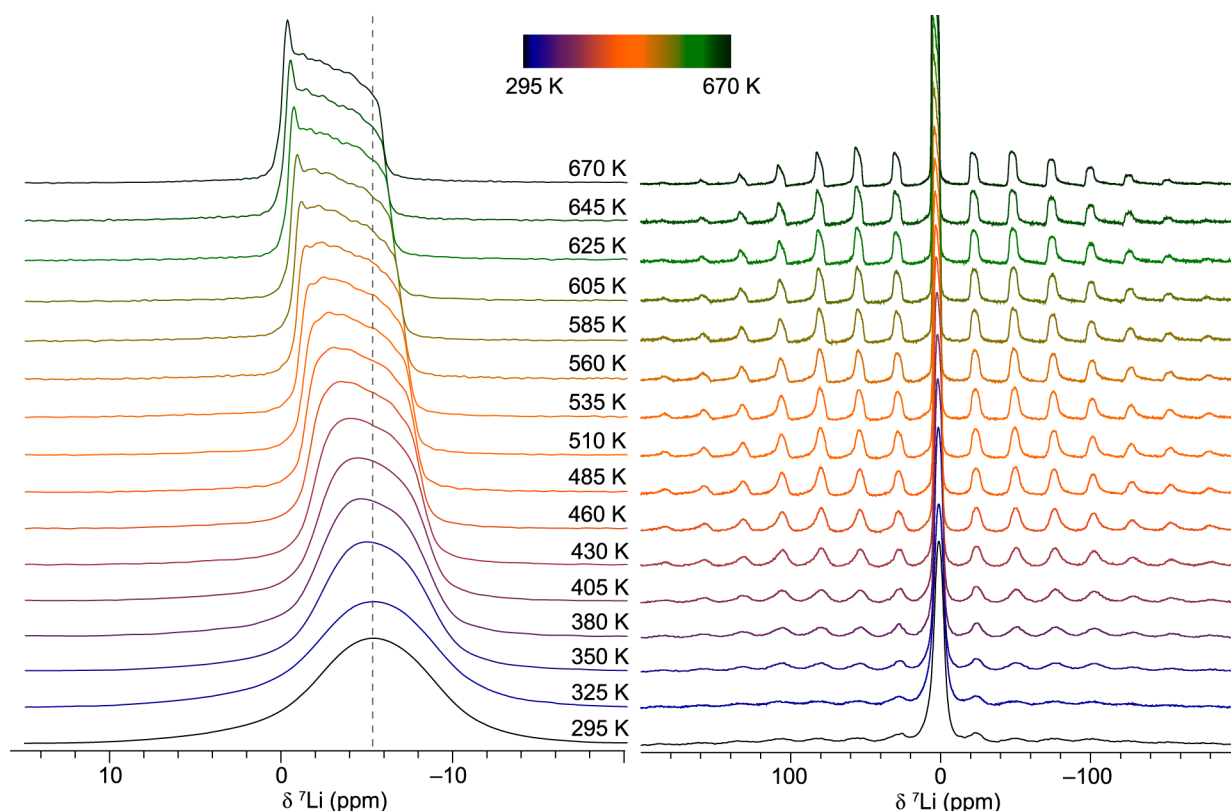
Figure 7. High-temperature ^7\text{Li} MAS NMR spectra of \text{Li}_{0.30}\text{TiNb}_2\text{O}_7 . The (a) central transition and (b) spinning sideband manifold are depicted as a function of temperature from 295 to 670 K (ascending). The dashed vertical line in (a) indicates the average shift in the ambient-temperature \delta(^7\text{Li}) spectrum. Spectra were recorded at 4 kHz MAS and 9.4 T. See also Figures S17–S22 in the Supporting Information.
