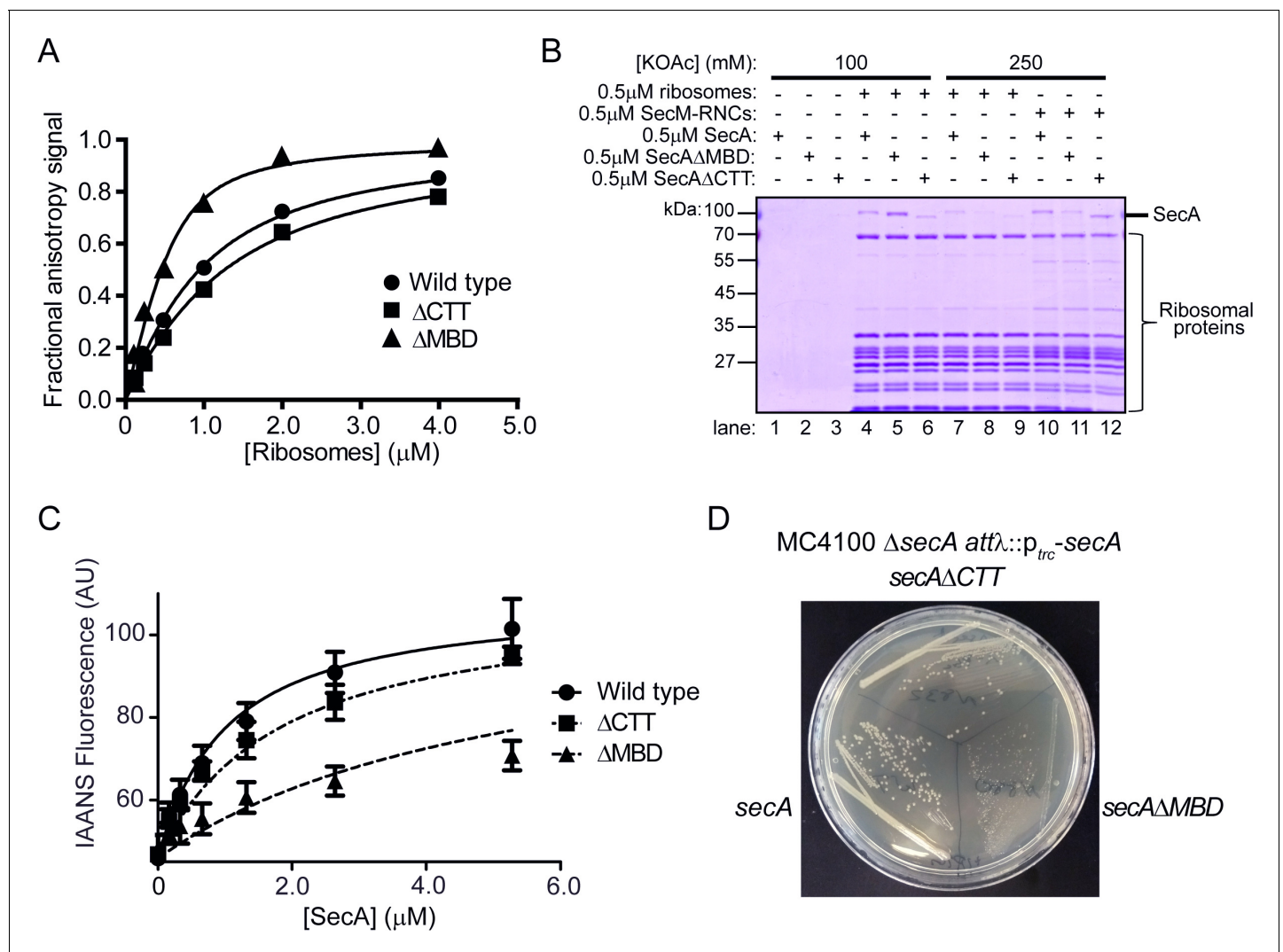
Figure 2. Effect of C-terminal truncations on SecA function in vitro and in vivo. (A) 900 nM Ru(bpy) 2 (dcbpy)-labelled SecA (Wild type; circles), SecA \Delta\text{MBD} ( \Delta\text{MBD} ; triangles) or SecA \Delta\text{CTT} ( \Delta\text{CTT} ; squares) was incubated in the presence of increasing concentrations of purified 70S ribosomes. Because error bars corresponding to one standard deviation obscured the symbols, they were omitted from the graph. The equilibrium dissociation constant ( K_D ) of the complex was determined by fitting the increase in fluorescence anisotropy from the Ru(bpy) 2 (dcbpy) (lines; Table 1 ). (B) 0.5 \mu\text{M} SecA, SecA \Delta\text{MBD} or SecA \Delta\text{CTT} was incubated in the absence (lanes 1–3) of ribosomes, in the presence of 0.5 \mu\text{M} vacant 70S ribosomes (lanes 4–9) or in the presence of 0.5 \mu\text{M} RNCs containing nascent SecM peptide (lanes 10–12). Where indicated, binding reactions were incubated in the presence of 100 mM (lanes 1–6) or 250 mM (lanes 7–12) potassium acetate (KOAc). Binding reactions were layered on a 30% sucrose cushion and ribosomes were sedimented through the sucrose cushion by ultracentrifugation. Ribosomal pellets were resolved by SDS-PAGE and stained by Coomassie. (C) 600 nM IAANS-VipB peptide was incubated with increasing concentrations of SecA (Wild type; circles), SecA \Delta\text{MBD} ( \Delta\text{MBD} ; triangles) or SecA \Delta\text{CTT} ( \Delta\text{CTT} ; squares). Confidence intervals represent one standard deviation. The K_D for the SecA-peptide complex was determined by fitting the increase in IAANS fluorescence upon binding to SecA (lines; Table 1 ). (D) Growth of strains producing SecA (DRH1119; bottom left), SecA \Delta\text{MBD} (DRH1120; bottom right) and SecA \Delta\text{CTT} (DRH1121; top) on LB plates containing 100 \mu\text{M} IPTG.
