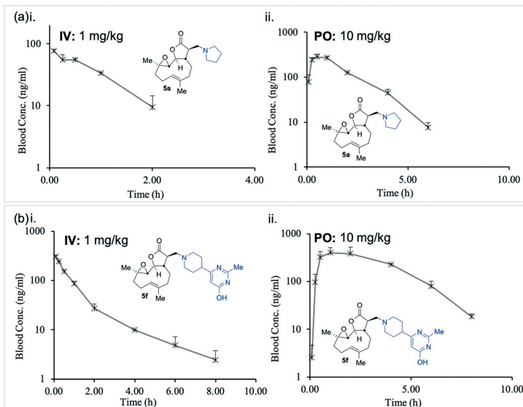
Fig. 4 Graphical representation of murine in vivo pharmacokinetic study, concentrations of 5a (a) and 5f (b) i. IV (1 mg kg -1 ); ii. PO (10 mg kg -1 ). Data summarised in Table 2.
