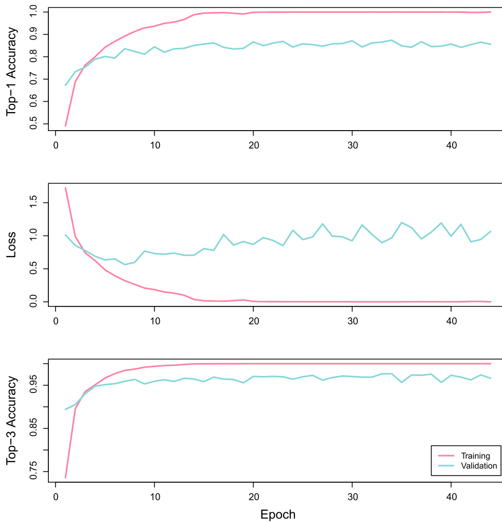
Figure 3. Plots showing evolution of top 1 accuracy, loss, and top 3 accuracy with epoch number during model training using the VGG16 CNN with an image size of 160 \times 160 pixels, a batch size of 200, 0.5 dropout regularization, a self-adjusting learning rate with an adjustment factor of 0.5, and early stopping with a patience of 10. A total of 44 epochs were completed before the early stopping algorithm stopped the run. The maximum top 1 training accuracy was 99.99%; the maximum top 1 validation accuracy was 87.41%; the minimum training loss was 0.0003; the minimum validation loss was 0.5638; the maximum top 3 training accuracy was 100%; and the maximum top 3 validation accuracy was 97.66%.
