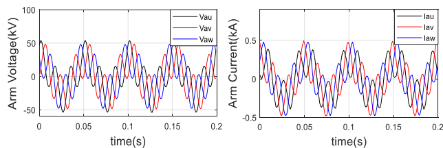
(c) M 3 C arm voltage (left) and current (right)
