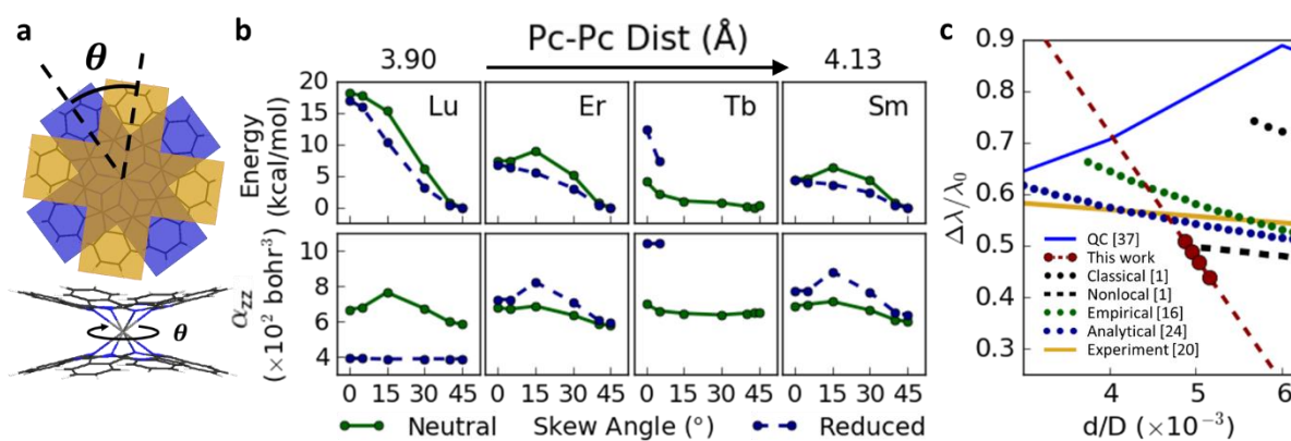
Figure 3. (a) Schematic of BPC molecule illustrating skew angle \theta . (b) Variation in relative energy (top) and polarizability (bottom) with change in skew angle for LnPc 2 and LnPc 2 - (Ln = Lu, Er, Tb, Sm). (c) Comparison of selected models from Table 1. QC = quantum corrected.
