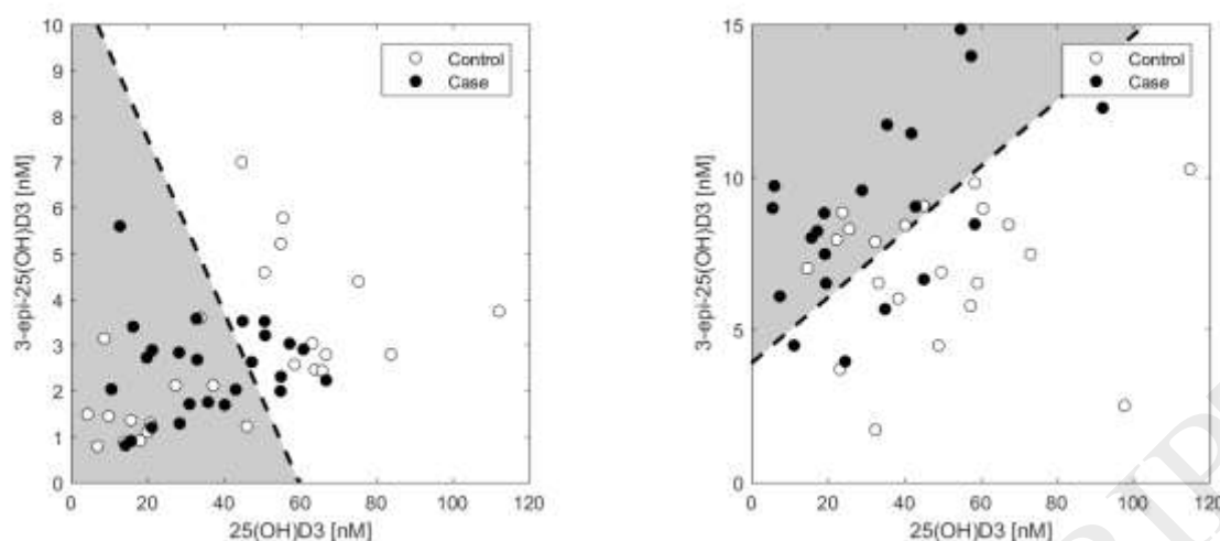
Figure 4: A two-dimensional linear classifier (dotted line) incorporating serum 3-epi-25(OH)D3 (y-axis) and 25(OH)D3 [nM] (x-axis) concentrations for the SCOPE (15 weeks of pregnancy) (left) and West Midlands (third trimester) data (right). The linear classifier classes serum data in the grey section as PET case and the remainder as being healthy pregnancies. False-positives and false-negatives are clearly visible and lead to a classification accuracy of only 56% (left) and 68% (right).
