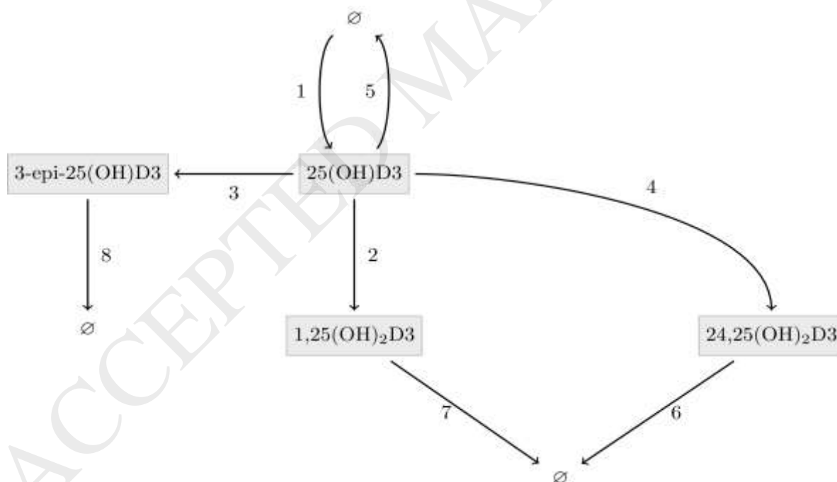
Figure 2: Network diagram of the reduced kinetic model for vitamin D metabolism. The network only contains chemicals with measured concentrations, 25-hydroxyvitamin D3 (25(OH)D3); C3-epimer 25-hydroxyvitamin D3 (3-epi-25(OH)D3); 1,25-dihydroxyvitamin D3
