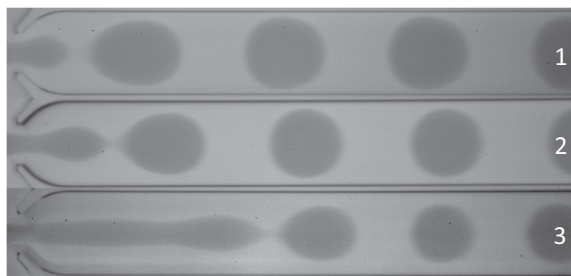
Fig. 6. Dependence of distance to the pinch-off point on surfactant concentration: 1 – surfactant-free aqueous solution, 2 – 5 mM of C_{12}TAB , 3 – 50 mM of C_{12}TAB . Q_c = Q_d = 0.1 mL/min.
