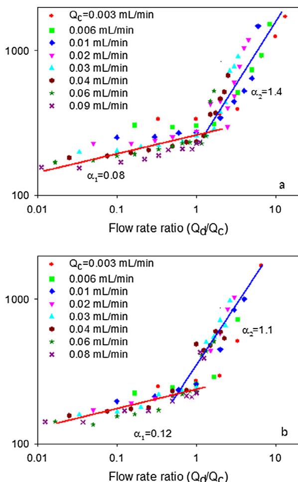
Fig. 10. Dependence of drop length of flow rate ratio for surfactant-free dispersed phase (a) and that containing 5 mM of C 16 TAB (b).
