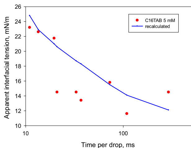
Fig. 8. Dynamic interfacial tension of 5 mM solution of C_{16} TAB at dripping to jetting transition. The points are obtained from Eq. (3). The line is obtained by mapping data for dynamic surface tension, see text for details.
