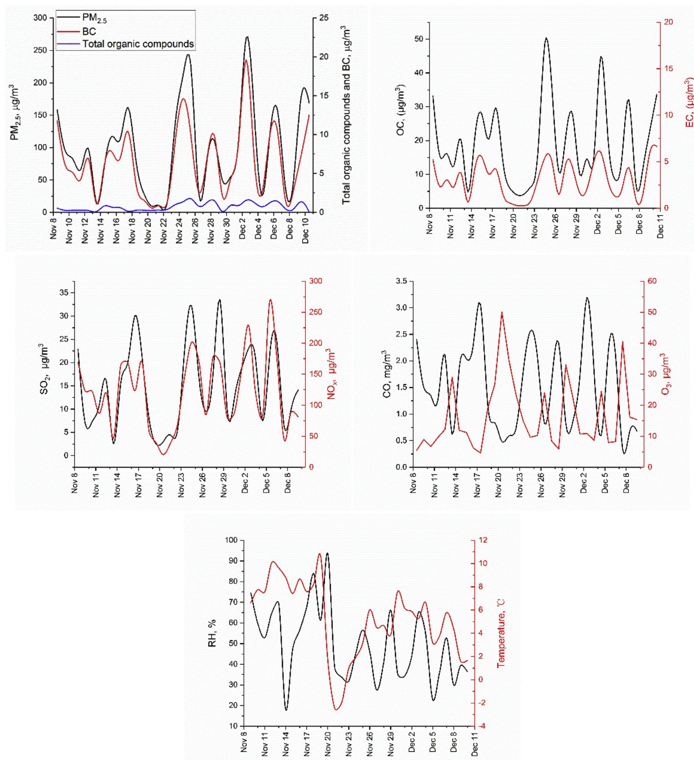
Fig. 2. Variations of particulate matter concentrations (PM 2.5 ) together with main meteorological variables, typical air pollution parameters and total mass concentration of 115 organic compounds during the sampling period.
