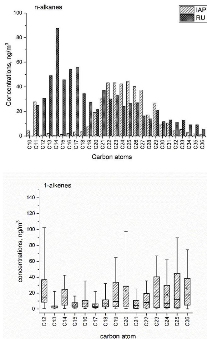
Fig. 3. Carbon number distributions and mass concentrations of PM 2.5 -bound n-alkanes and n-alkenes at IAP (Beijing) and RU (London).
