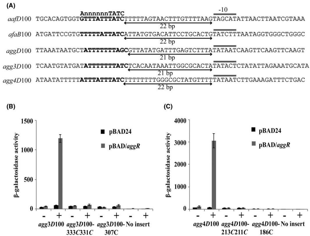
Fig. 5. Analysis of EAEC 55989 agg3D100 and EAEC C1010-00 agg4D100 promoter fragments.
