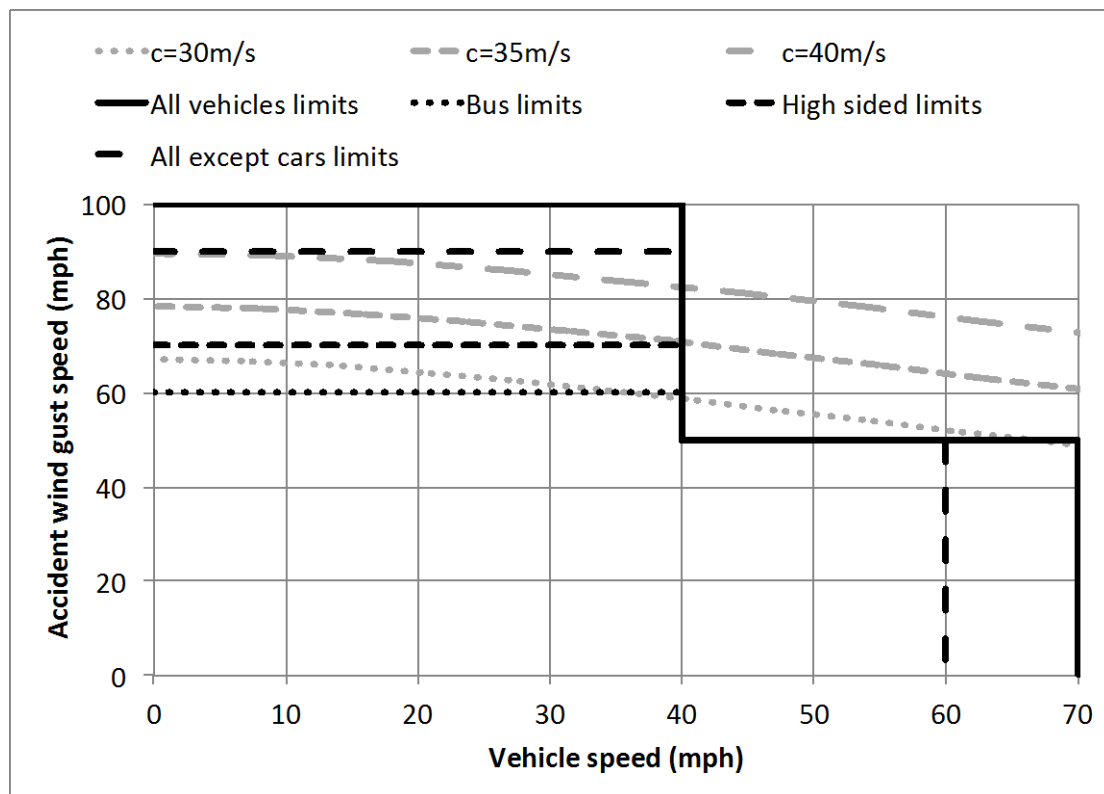
Figure 5. Minimum overturning wind speed for all wind directions against vehicle speed for values of c of 30, 35 and 40m/s and Queensferry Bridge limits for different vehicle categories (vertical lines at 60 and 70mph indicate national speed limits for different vehicle classes)
