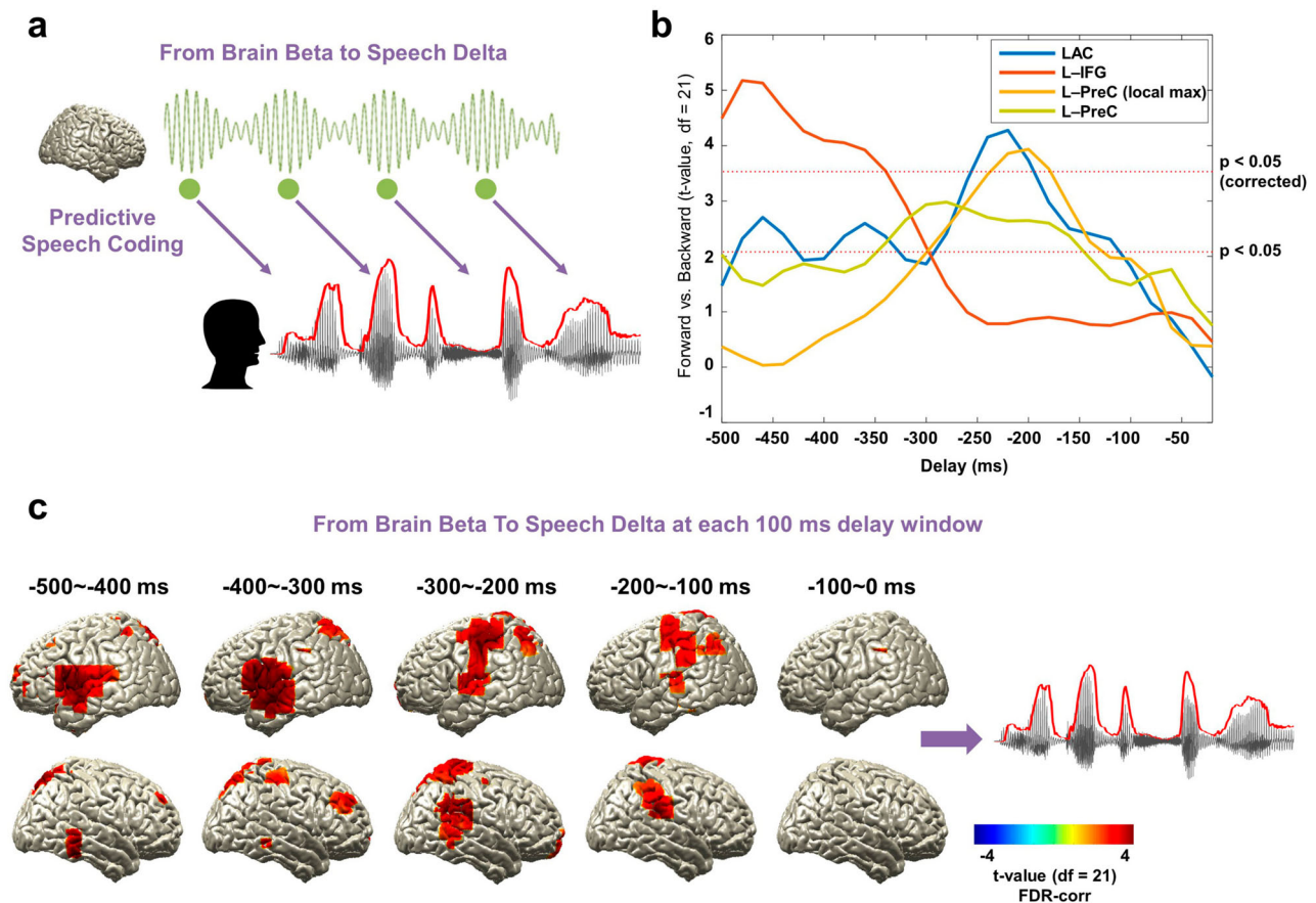
Figure 4. Beta rhythms and the prediction of upcoming speech. (a) A schematic figure for directed causal analysis: TE from brain beta power to speech delta phase (negative delays between speech-brain). TE computation was performed for each condition (forward played and backward played) at each voxel from 20 to 500 ms in 20 ms steps and compared statistically between conditions. Green line represents beta rhythm in the brain and each circle represents a certain point in time. (b) TE values are averaged within each ROI from the AAL atlas and compared statistically between conditions. T -values are shown in each ROI: left primary auditory cortex (Heschl gyrus) (blue line), left IFG (orange line), and left precentral gyrus (both at local maximum coordinate (yellow line) and whole precentral gyrus ROI (light green line)). Statistical significance was shown with two red lines depicting t -values by paired t -test (upper red line: t_{21} = 3.53 , p < 0.05 , corrected; bottom red line: t_{21} = 2.08 , p < 0.05 , uncorrected). Left-lateralised predictions by beta power were observed (see Supplementary Figure 2). (c) Statistical contrast maps of averaged across 100 ms windows show that intelligibility-dependent prediction first engages left inferior frontal gyrus about 300–500 ms prior to the speech followed by left precentral gyrus and left primary auditory area 200–300 ms prior to the speech ( p < 0.05 , FDR-corrected).
