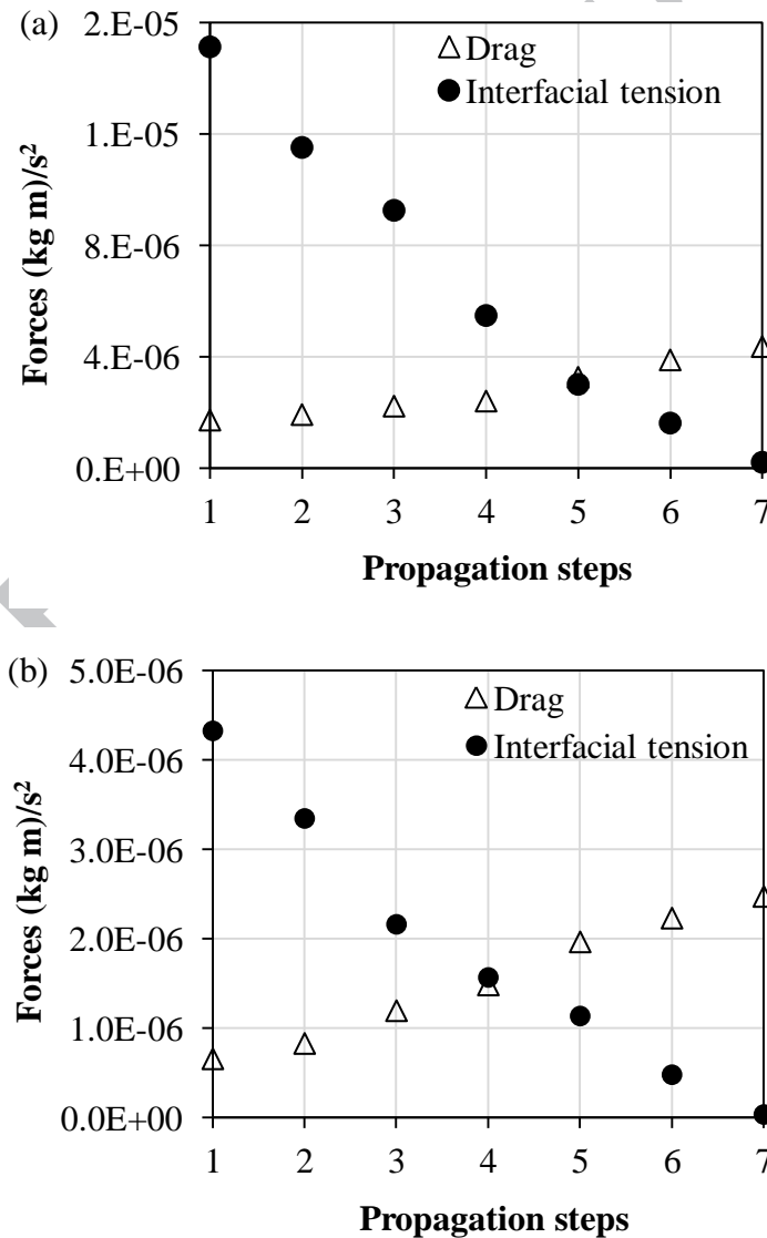
Figure 14: Forces during the formation of (a) surfactant-free and (b) C_{12}TAB surfactant-laden droplets. Q_D = 0.01 cm 3 /min and Q_C = 0.08 cm 3 /min.
