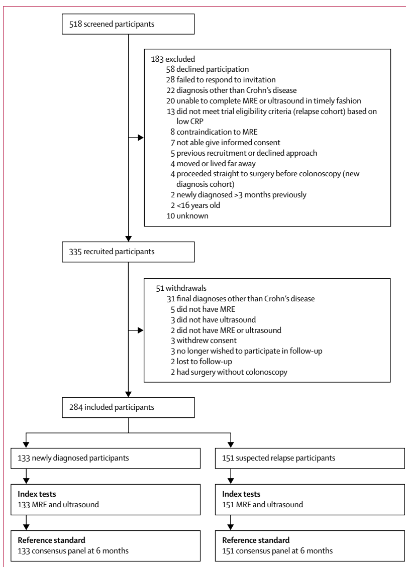
Figure 1: Trial profile
