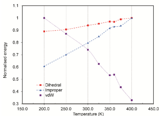
Figure 7. Normalised dihedral, improper and van der Waals (vdW) energies as a function of temperature. There is a change in the gradient at the temperature about 350K, which is related to the T_g .
