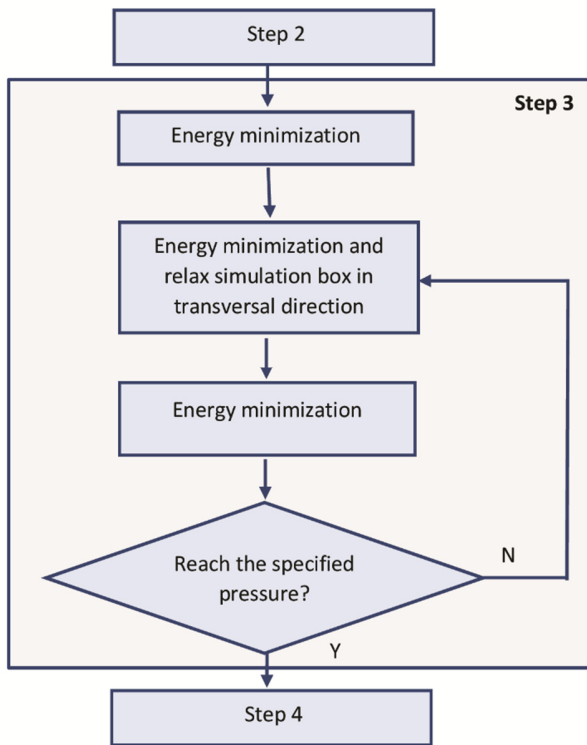
Figure 2. Step 3 may be combined with additional energy minimization processes and repeated several times in order to gradually change the pressure to the specified value.
