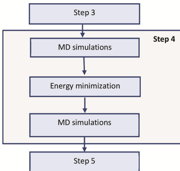
Figure 3. An energy minimization process may be performed in between two MD simulations in step 4 to accelerate the rate at which the equilibrium state is achieved.
