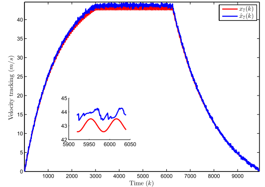
Fig. 7. The velocity tracking trajectories \tilde{x}_7(k) and \hat{x}_7(k) .
