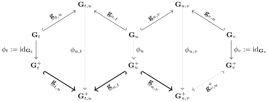
Figure 2. The case (u,v) \in S and (v,u) \notin S .
