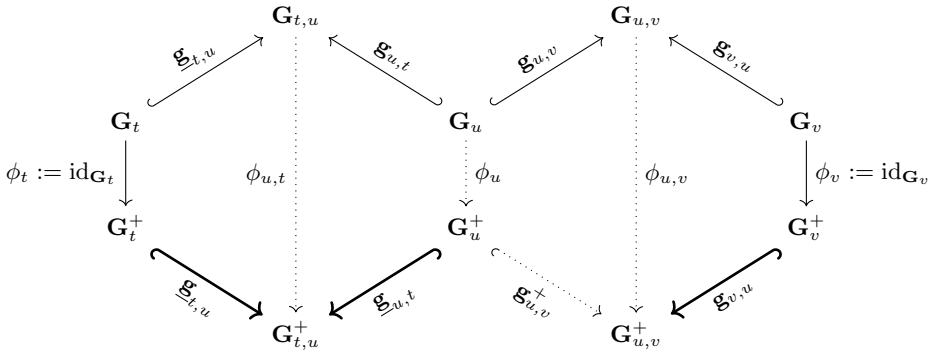
Figure 3. The case (u,v) \notin S and (v,u) \in S .
