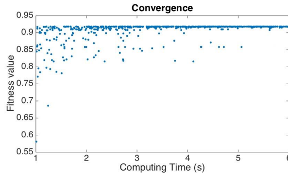
Fig.14.The convergence
