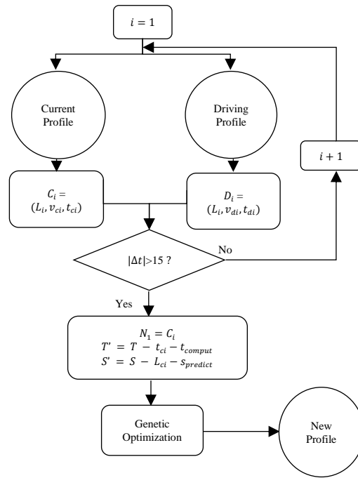
Fig.7.The dynamic programming
