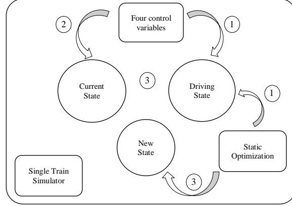
Fig.6.The procedure of dynamic optimization
