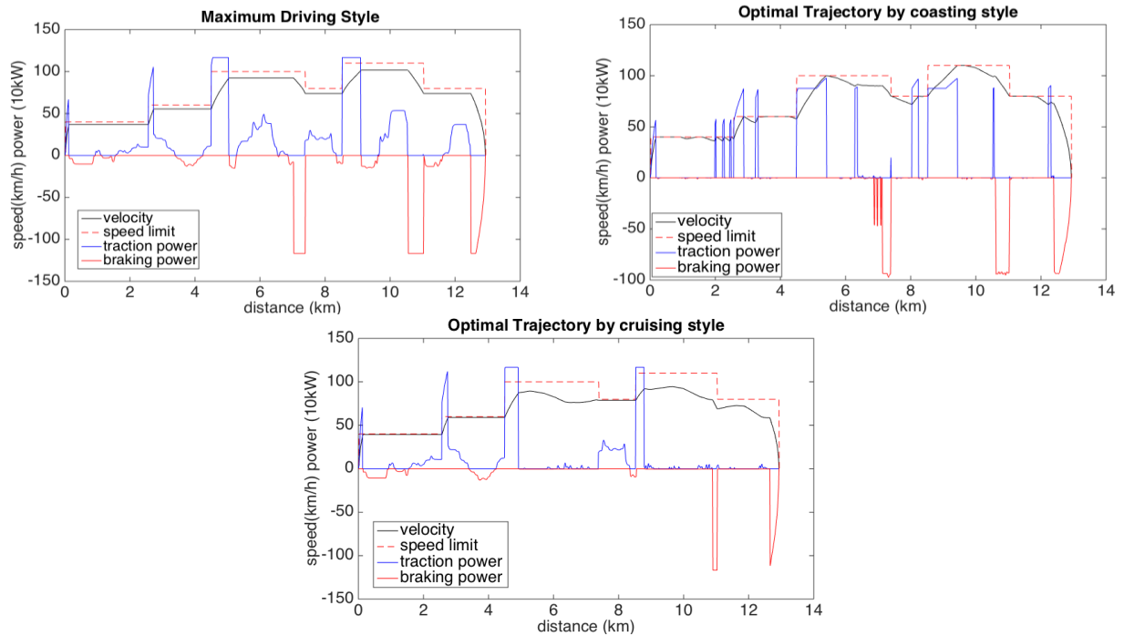
Fig.12. Static optimization for the simulated trajectory in diving styles (a) Without optimization (b) Optimal coasting style (c) Optimal cruising + coasting style
