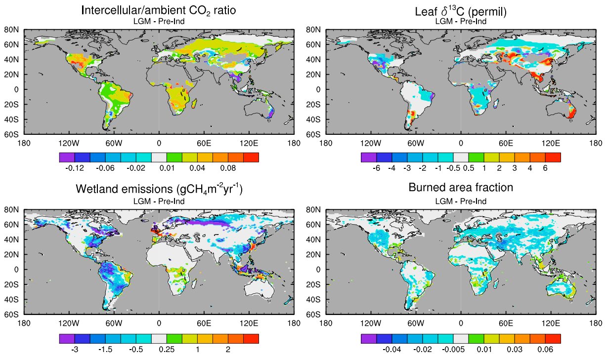
Figure 2. HadGEM2-ES simulated Last Glacial Maximum minus preindustrial anomalies in intercellular/ambient CO 2 ratio, leaf \delta^{13}\text{C} (this study) and wetland CH 4 emissions, and burned area fraction (from H17). The CO 2 ratios and \delta^{13}\text{C} fields are masked over desert and ice regions. Emissions and burned area anomalies are shown over new land points and where ice sheets change to clarify the role of geographical differences between the two time periods.
