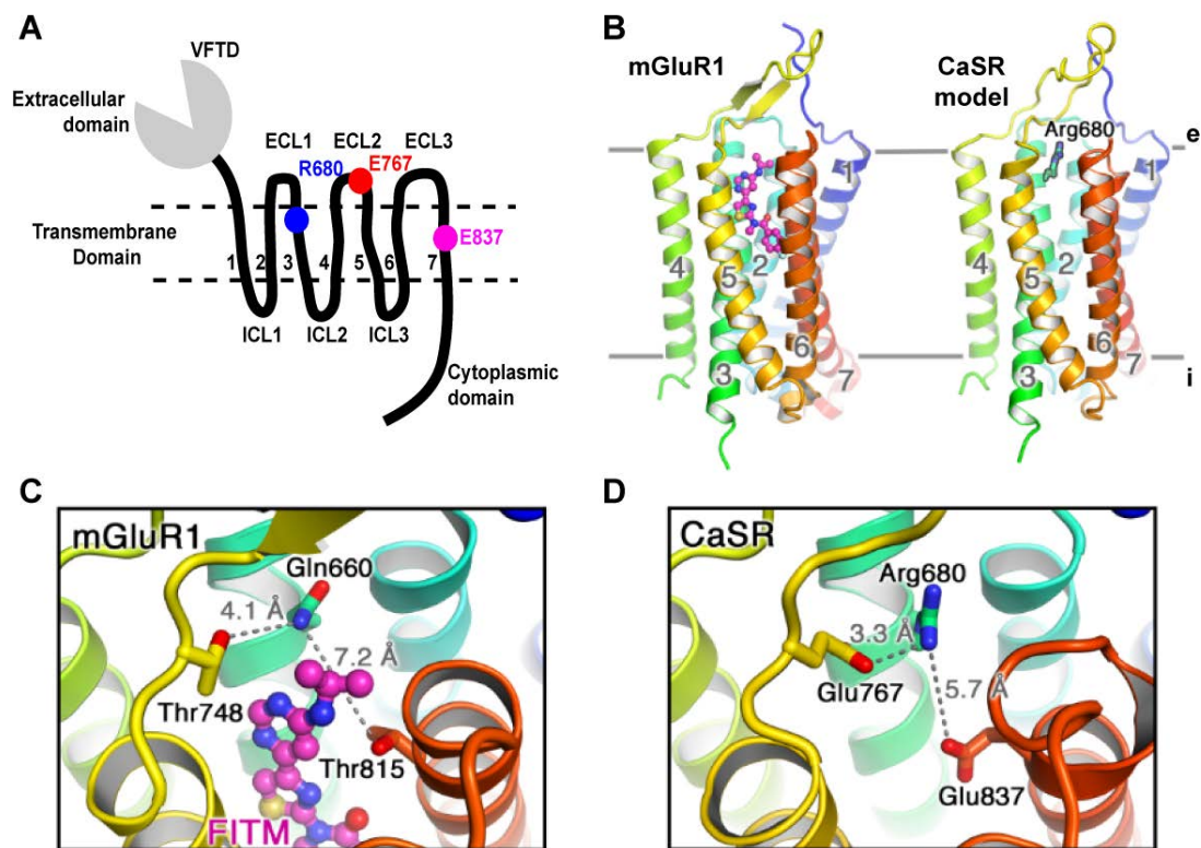
Fig. 7. The Arg 680 residue of CaSR forms a salt bridge with either Glu 767 or Glu 837
