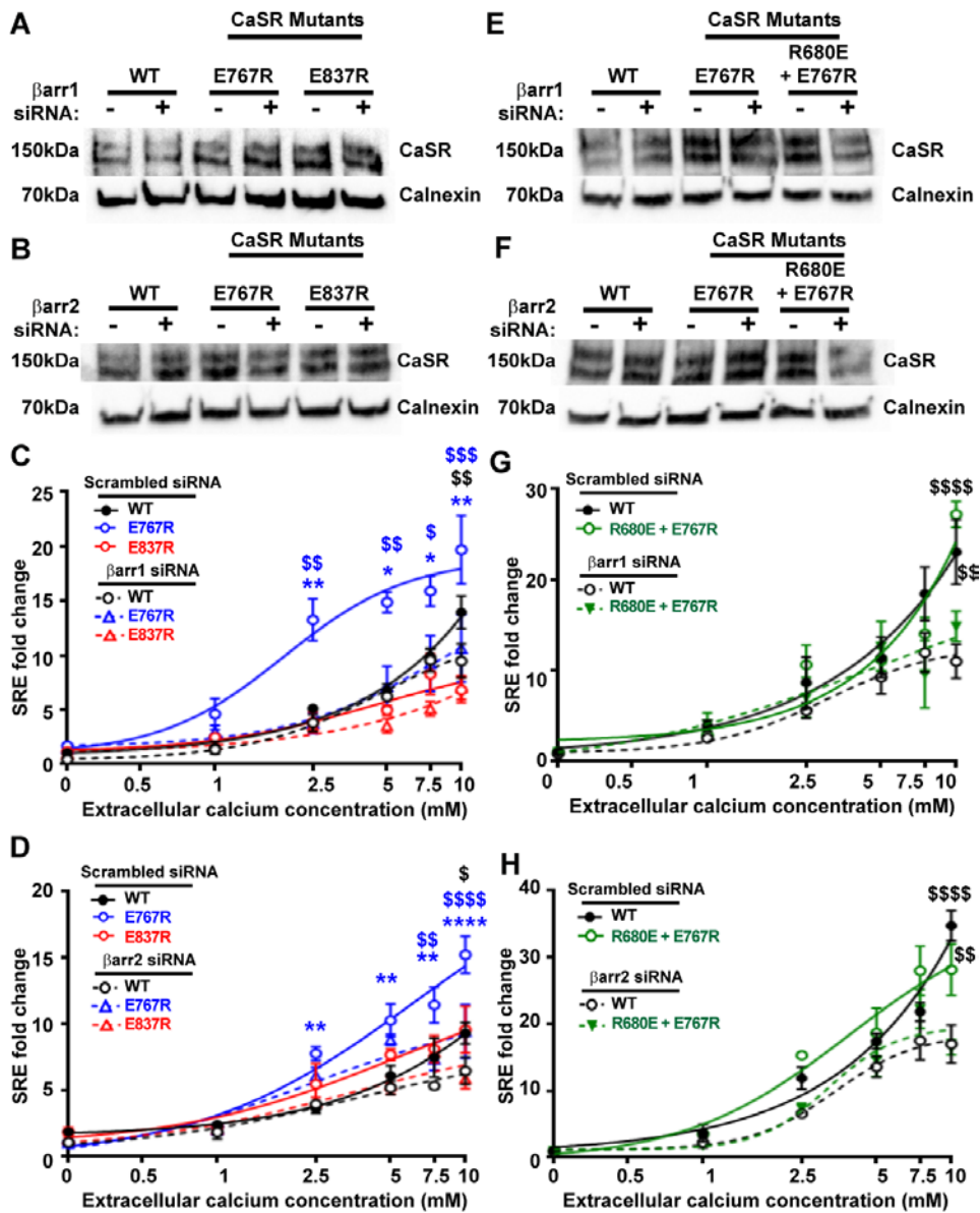
Fig. 8. Disruption of the Arg 680 -Glu 767 salt bridge leads to increased \beta -arrestin-mediated MAPK signaling
