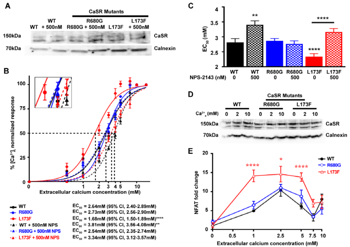
Fig. 2. The CaSR R680G mutation does not affect intracellular Ca 2+ signaling
