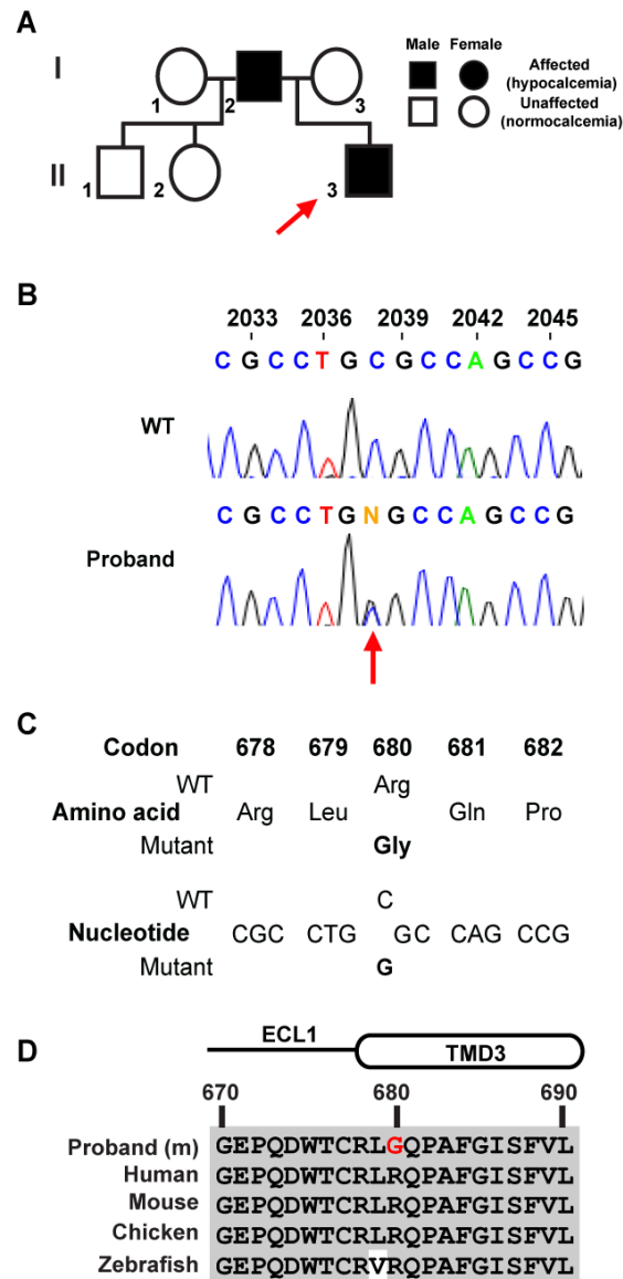
Fig. 1. Identification of an R680G CaSR mutation in a family with autosomal dominant hypocalcemia type 1 (ADH1)
