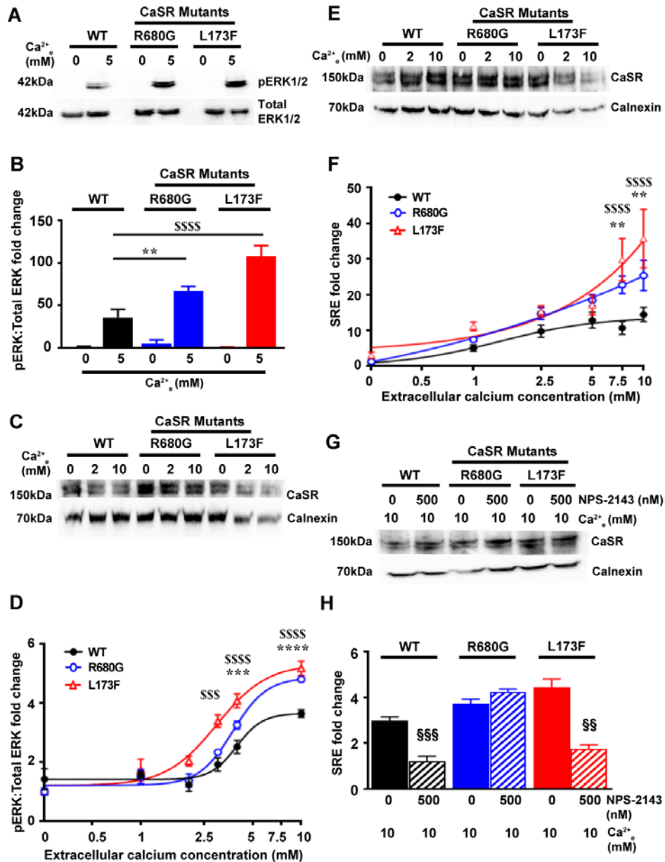
Fig. 3. The CaSR R680G mutation increases downstream MAPK signaling
