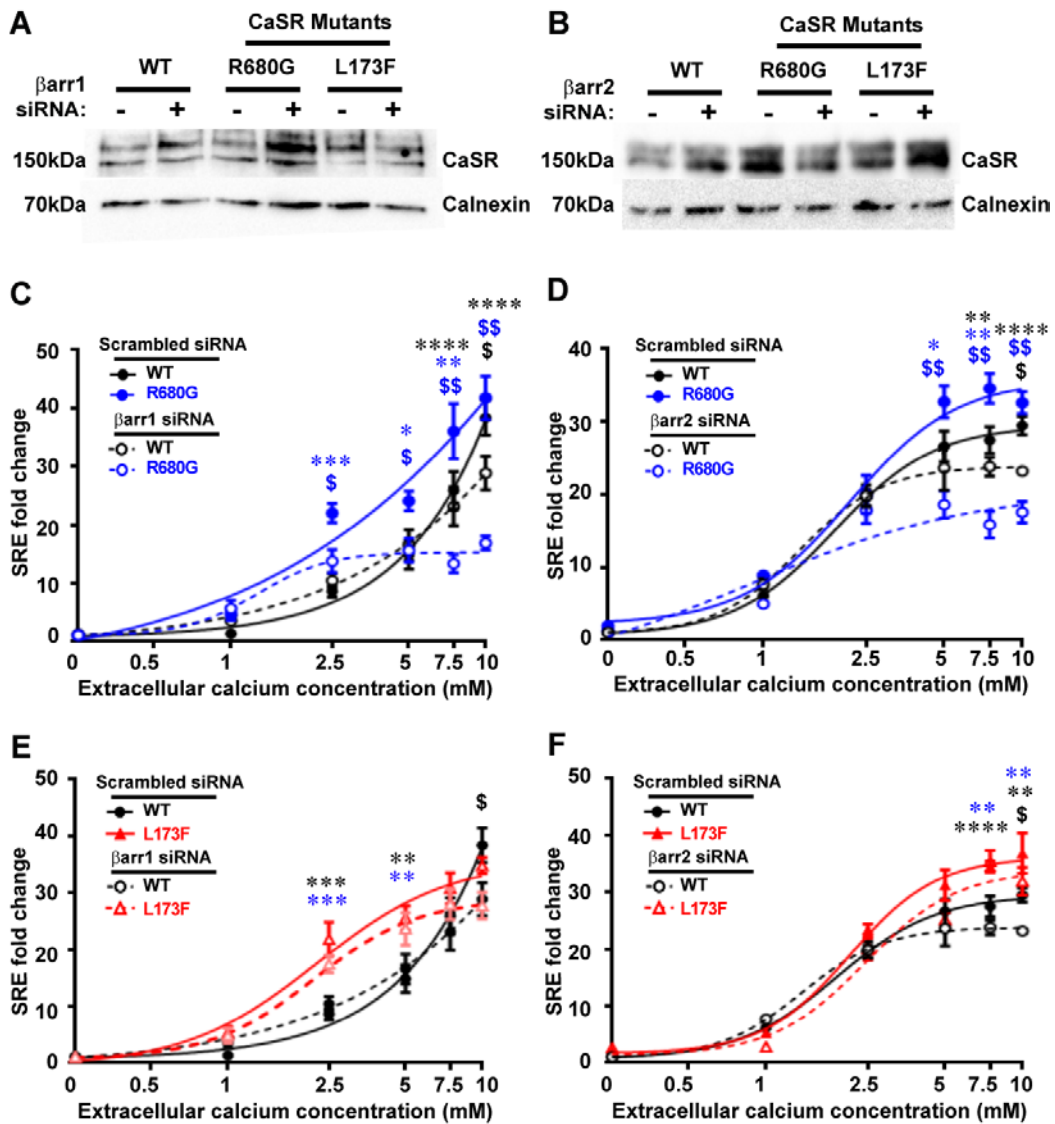
Fig. 6. Increased MAPK responses in cells expressing CaSR R680G involve a G-protein-independent, \beta -arrestin-dependent pathway
