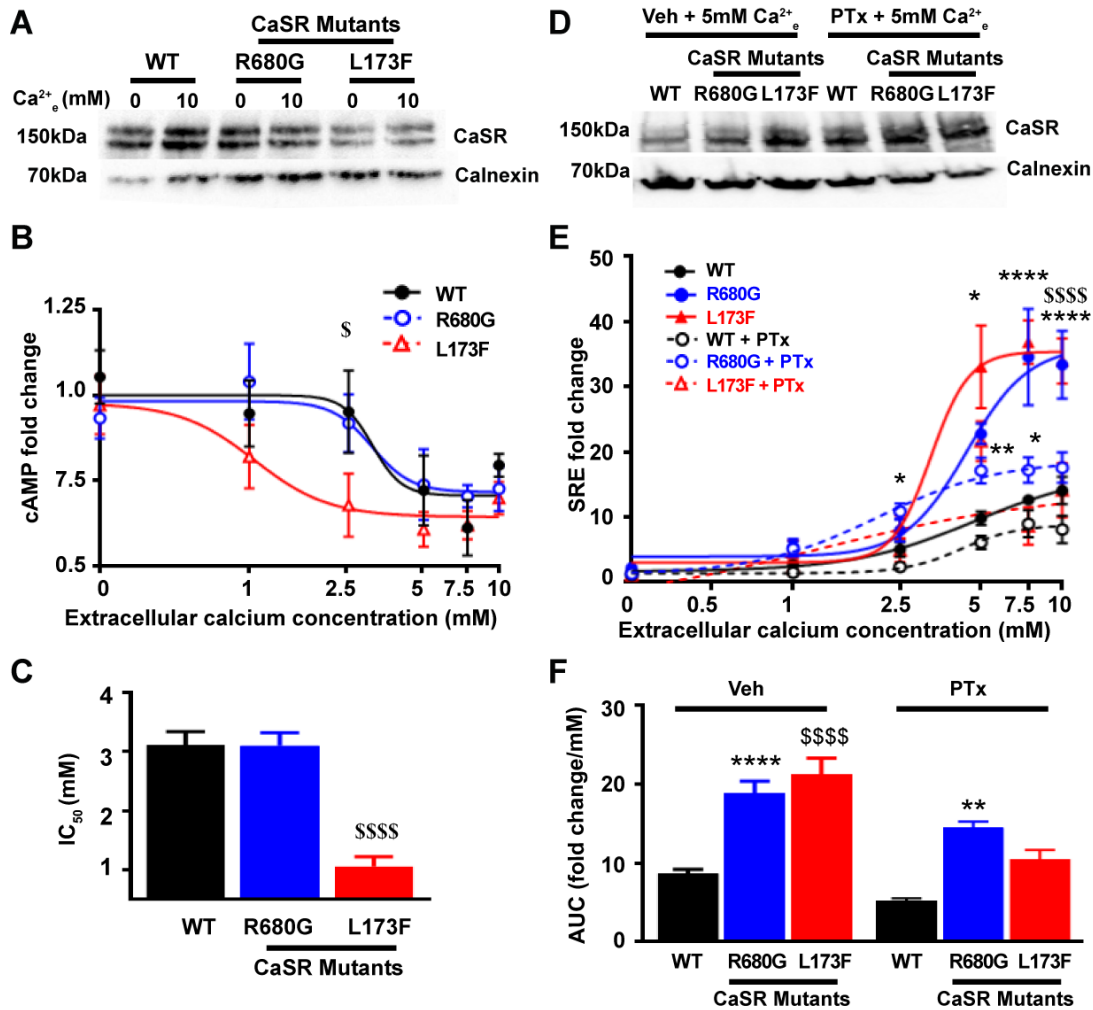
Fig. 5. The CaSR R680G mutation does not affect G_{i/o} -mediated signaling
