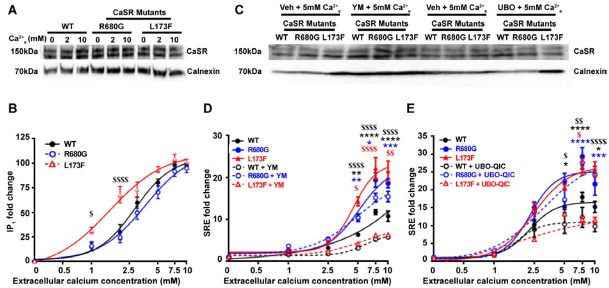
Fig. 4. The CaSR R680G mutation does not affect G_{q/11} -mediated signaling
