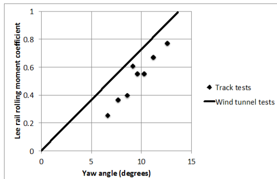
(d) TRANSAERO experiments - lee rail rolling moment results (from Matschke and Heine 2002 - redrawn). Note that the wind tunnel results are not from an identical train and are extrapolated from higher yaw angle values.
