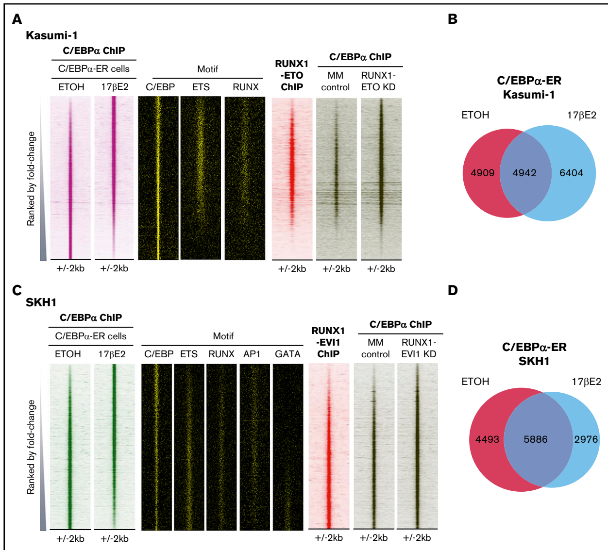
Figure 4. Comparison of C/EBP \alpha binding after induction and after RUNX1-ETO or RUNX1-EVI1 knockdown. (A,C) ChIP-seq of C/EBP \alpha after E2 induction in (A) C/EBP \alpha -ER Kasumi-1 or (C) C/EBP \alpha -ER SKH1 cells. Peaks are ranked in order of decreasing relative DNA sequence tag count for peaks in control cells. Aligned to these coordinates are the indicated motifs, ChIP-seq sequences for either RUNX1-ETO (in Kasumi-1) or RUNX1-EVI1 (in SKH1), and C/EBP \alpha ChIP-seq after either control siRNA or CBF fusion knockdown in the respective cell lines. Overlap of C/EBP \alpha ChIP-seq peaks in (B) C/EBP \alpha -ER Kasumi-1 or (D) C/EBP \alpha -ER SKH1 cells after E2 and ethanol treatment.
