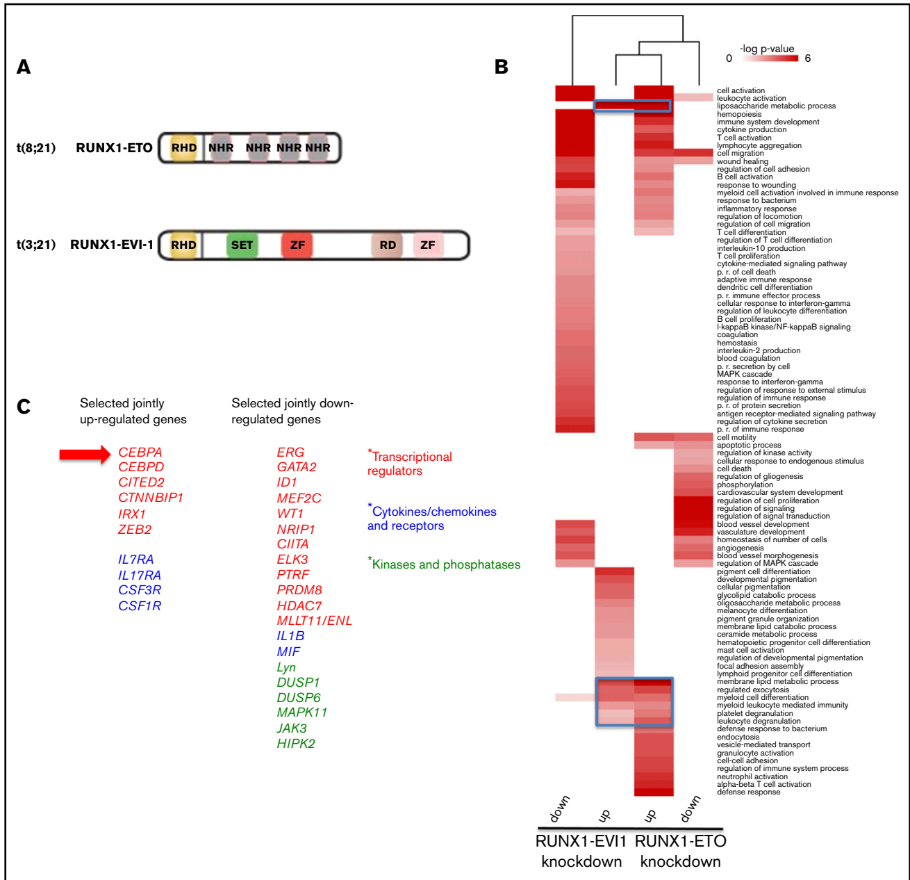
Figure 1. Response to knockdown of RUNX1-EVI-1 and RUNX1-ETO converges on a C/EBP \alpha -driven differentiation program. (A) Structure of RUNX1-EVI1 and RUNX1-ETO. NHR, neryv homology region; RD, proline-rich repressive domain; RHD, Runt homology domain; SET, Su(var)3-9 and enhancer of zeste and trithorax; ZF, zinc finger domain. (B) Hierarchical clustering of GO terms for upregulated or downregulated genes (1.5-fold difference) after either RUNX1-EVI1 or RUNX1-ETO knockdown compared with control siRNA. Expression after treatment was measured after 10 days in SKH-1 cells or 4 days in Kasumi-1 cells. The blue box identifies GO terms commonly upregulated after knockdown of both RUNX1-ETO and RUNX1-EVI1. (C) Selected examples of upregulated or downregulated genes.
