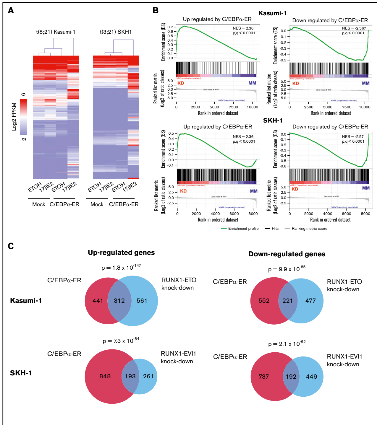
Figure 3. C/EBP \alpha induction and CBF fusion protein knockdown induce similar changes in the transcriptional program. (A) Hierarchical clustering of RNA-seq data by log 2 fold FPKM (fragments per kilobase of transcripts per million mapped reads) values of genes differentially expressed (twofold change) after C/EBP \alpha induction by E2 or vehicle as indicated (4 days for Kasumi-1 and 2 days for SKH-1). (B) Comparison of up- and downregulated genes after C/EBP \alpha -ER induction in Kasumi-1 and SKH1 cells with genes changing expression after RUNX1-ETO and RUNX1-EV1 knockdown (KD) or control siRNA treatment (MM). (C) Number of genes changing expression at least 1.5-fold after C/EBP \alpha induction in Kasumi-1 and SKH1 cells as compared with RUNX1-EV1 or RUNX1-ETO knockdown. The P values in panel C were calculated with Fisher's exact test using the total set of genes expressed in each condition as the background.
