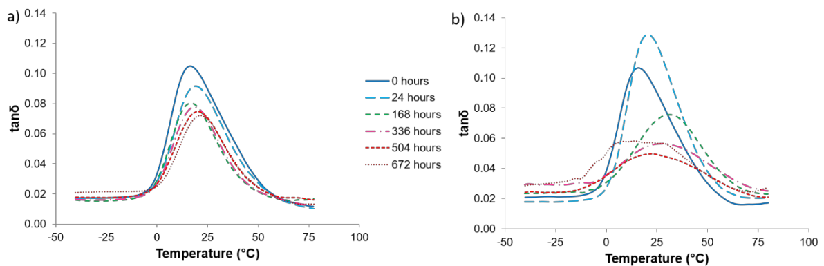
Figure 4: DMTA \tan\delta curves during storage at a) 20 °C and b) 150 °C
