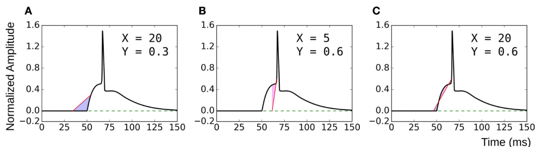
FIGURE 9 | Choice of parameters X and Y. (A) and (B) are examples of inappropriate choices of X and Y. (C) covers both the entire height and width of the AP foot and is consequently a good choice of parameter values.
