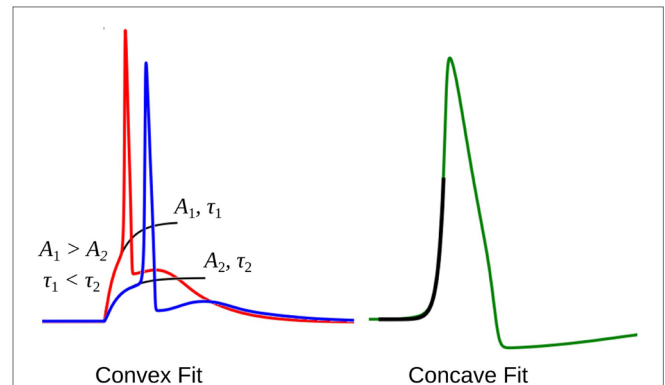
FIGURE 6 | The exponential fit for two convex footed APs (left) and one concave footed AP (right). The comparison of the fitting parameters corresponding to the two convex foots are also shown. See text for details.
