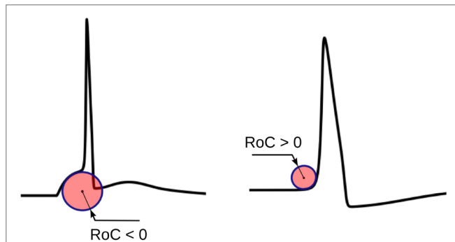
FIGURE 5 | The physical significance of the radius of curvature (RoC). The RoC values measured at convex foot is negative and that in concave foot is positive. These signs are flipped to match the convention followed in other techniques.
