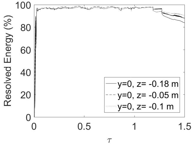
Figure 9: Percentage of turbulence kinetic energy that is directly resolved at COT for z=-0.18 m, -0.1 m and -0.05 m.
