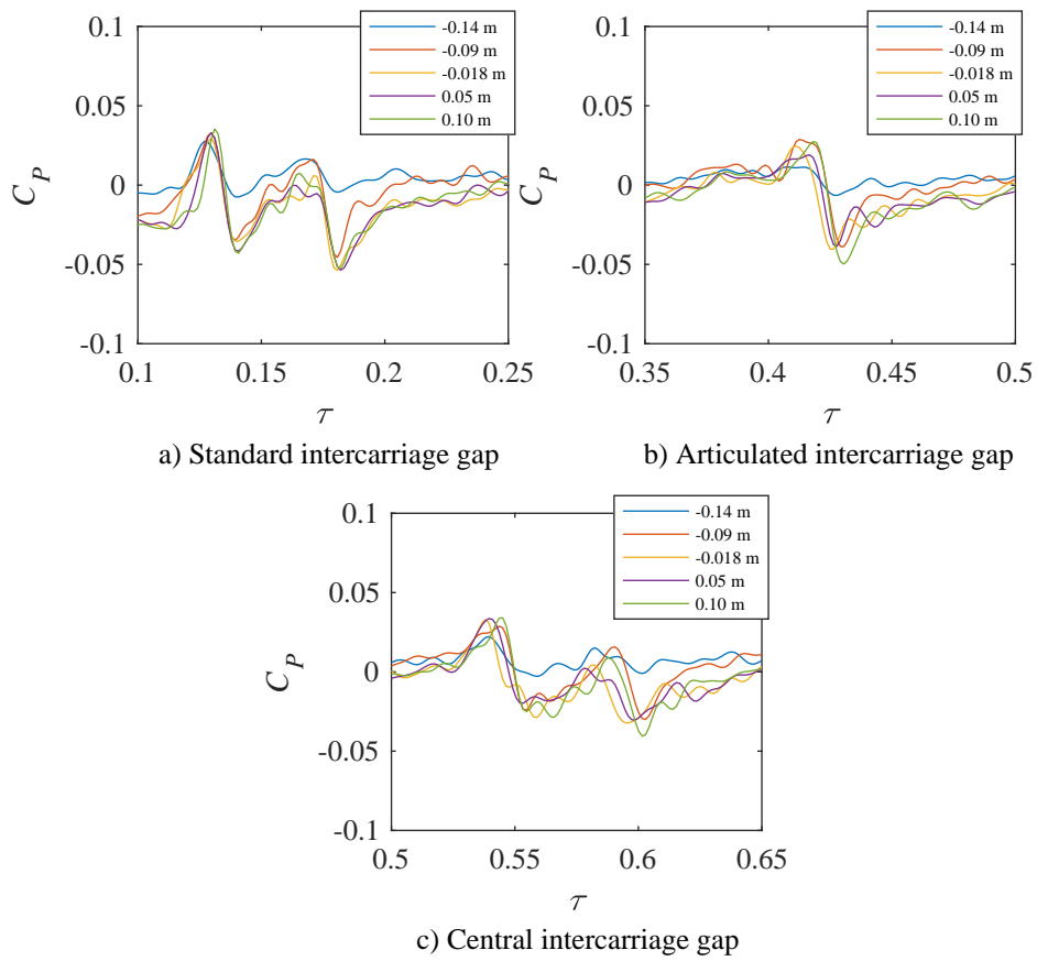
Figure 13: Model-scale individual bogie results for coefficient of pressure C_P measured at 0 m from centre of track.
