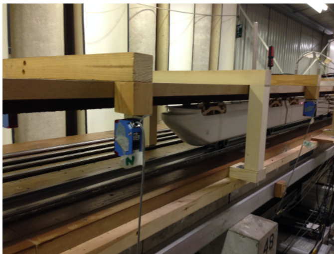
Figure 3: The upside-down ground plain with Class 373 Eurostar model and measuring instrumentation.
