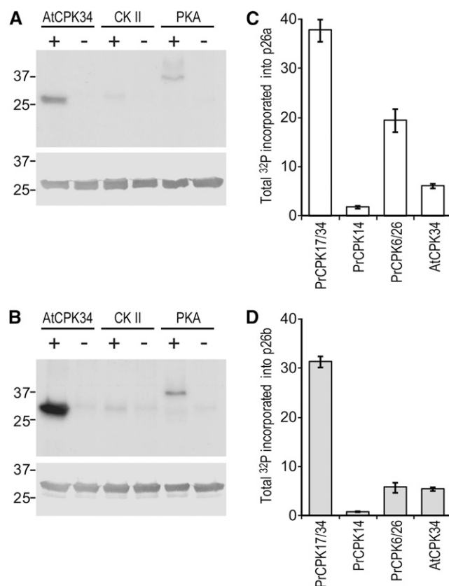
Figure 2. Phosphorylation of recombinant p26 by CPKs in vitro. A and B, Incorporation of ^{32}\text{P} into p26 after in vitro kinase assays using recombinant AtCPK34, CKII, or PKA with recombinant p26a (A) and p26b (B). Top gels are autoradiographs showing ^{32}\text{P} incorporation (total pmol), and bottom gels are western blots to show equal loading of protein. C and D, Incorporation of ^{32}\text{P} into p26a (C) and p26b (D) during in vitro phosphorylation using PrCPK17/34, PrCPK14, PrCPK6/26, or AtCPK34. Values are means \pm SE ( n = 3 ).
