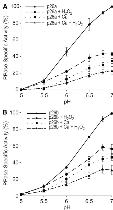
Figure 6. pH further reduces PPase activity in the presence of \text{Ca}^{2+} and \text{H}_2\text{O}_2 . Recombinant sPPase p26a (A) and p26b (B) enzymes were assayed for PPase activity (diamonds) and in the presence of \text{CaCl}_2 (squares), \text{H}_2\text{O}_2 (circles), and \text{CaCl}_2 + \text{H}_2\text{O}_2 (triangles) at several pH levels. The activity for each was reduced further by lowered pH. Values are means \pm SE ( n = 5 for p26a and n = 3 for p26b).
