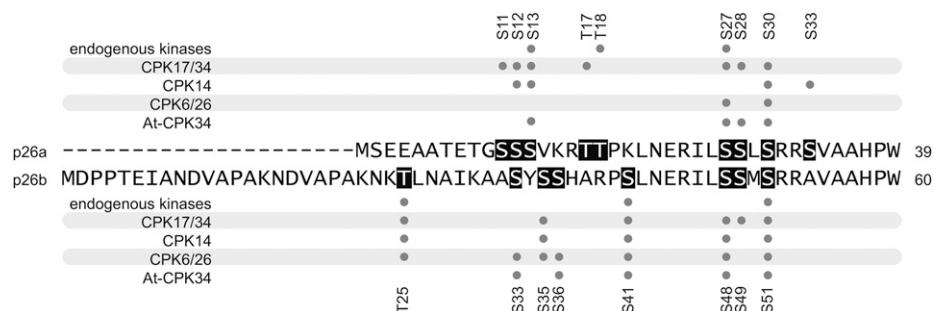
Figure 3. Phosphorylation sites identified by LC-MS/MS in p26 sPPase proteins phosphorylated by CPKs. The sequence alignment of the N-terminal regions of the p26 sPPase proteins is annotated to indicate phosphorylations by individual recombinant kinases and whole pollen extract. S/T, Phosphorylated residues.
