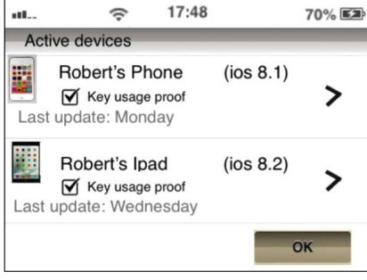
Fig. 3. An example of envisaged GUI that presents the table (D_i, t_i) for i = \{1, 2\} to Robert. The ticked box against the “key usage proof” indicates that the proofs about the usage statement (e.g., last update time) have been cryptographically verified.
