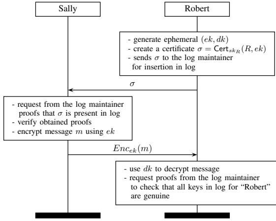
Fig. 2. The basic DECIM protocol. Robert has a pair (sk_R, vk_R) of long term keys for signature signing and verification. He generates an ephemeral key pair (ek, dk) for encryption, creates the certificate \sigma = \text{Cert}_{sk_R}(R, ek) on ek , and sends the certificate to the log maintainer for insertion into the public log. Meanwhile, Robert also sends the certificate to Sally. After receiving \sigma , Sally requests from the log maintainer proofs that the certificate is present in the log. If the proof is valid, Sally sends a message m to Robert encrypted with ek . Robert requests proofs from the log maintainer to enable him to verify whether the log contains signatures that he did not generate.
