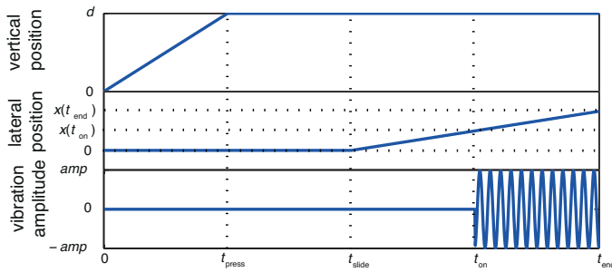
Fig. 6: Loading conditions for the FE examples.
