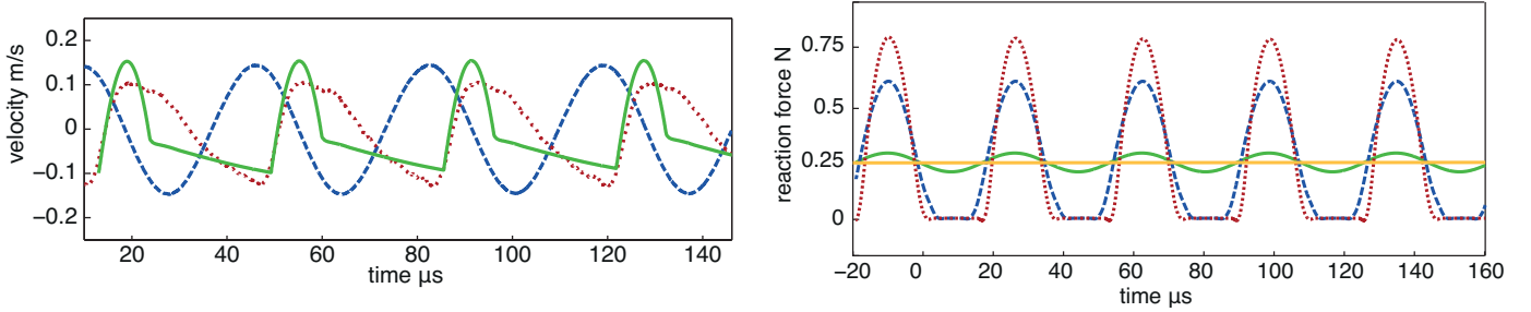
Fig. 5: Comparison between simulated (continuous green line) and measured (dotted red line) velocities of the finger print ridge (dry case) for a vibrational amplitude of 1.35 \mu\text{m} ; the plate velocity is plotted as a dashed blue line; the velocity corresponds to one node at the base of the ridge.
