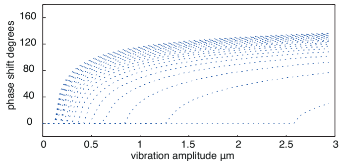
Fig. 11: Phase shift calculated using the spring-slider model for spring stiffnesses in the range from 0.2 (lower line) - 4 MN/m (upper line) for an applied normal force of 0.5 N.
