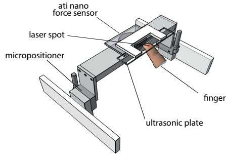
Fig. 1: Schematic diagram of the equipment used to measure the contact time between a finger pad and vibrating plate. The finger is inclined at an angle of 45^\circ to the plate and the focus spot is visible on the skin surface.
