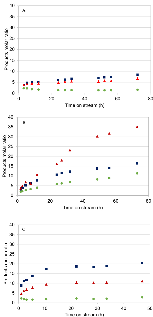
Fig. 7. Molar ratio of (blue square) p -cresol (1)/hydrogenated p -cresol products (6–7), (red triangle) m -cresol (5)/hydrogenated m -cresol products (8–9) and (green dot) methylcatechol (3)/hydrogenated methylcatechols products (10–11) as function of the time on stream at 300 °C, 2.5 WHSV, 4 bar of H 2 and H 2 /PMG molar ratio of 15 [A: 1.55%Pt/SiO 2 (A); B: 2.5%Rh/SiO 2 (JM); C: 2.5%Rh/SiO 2 (A)]. (For interpretation of the references to colour in this figure legend, the reader is referred to the web version of this article.)
