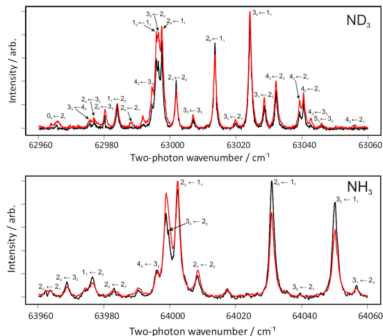
Figure 2: Experimental (2+1) REMPI spectra of \text{ND}_3 and \text{NH}_3 , recorded with the laser polarisation axis aligned parallel (black) and perpendicular (red) to the electric field axis. Each of the four spectra are normalised to the total integrated intensity in the spectral region, and transitions are labelled as J_K .
