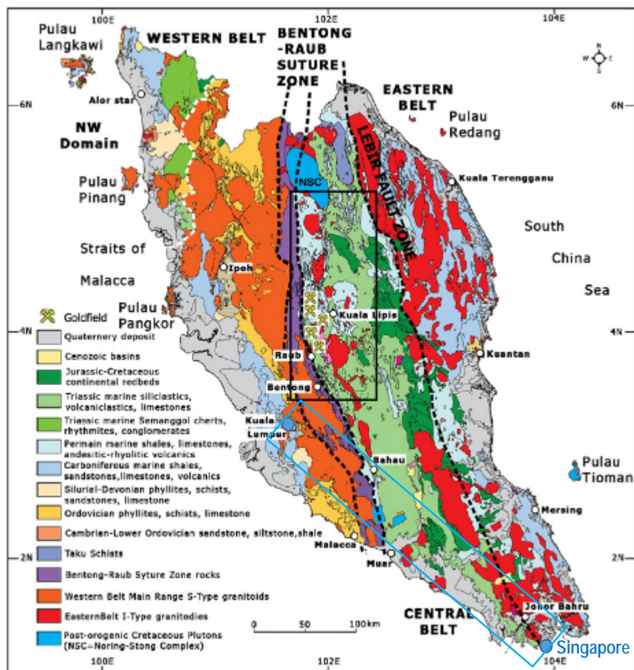
Figure 6. Geology Map of Peninsular Malaysia, modified from [25].
