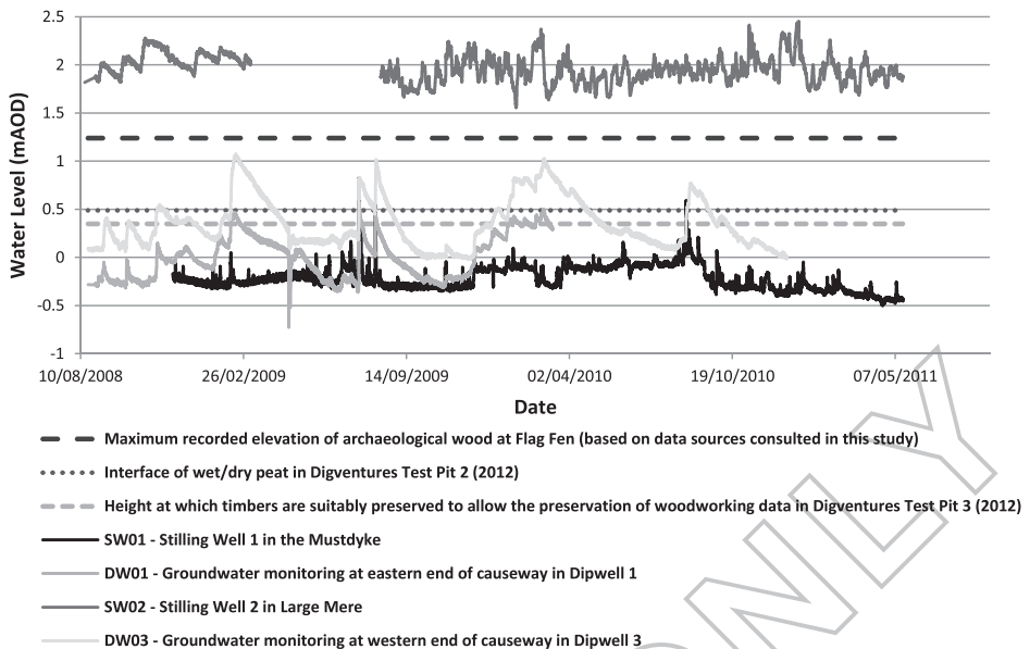
FIGURE 5 Summary of groundwater level monitoring at Flag Fen.
