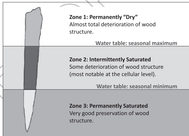
FIGURE 2 Three-zone model illustrating the link between groundwater levels and the preservation of archaeological wood. After Chapman & Cheetham (2002)
