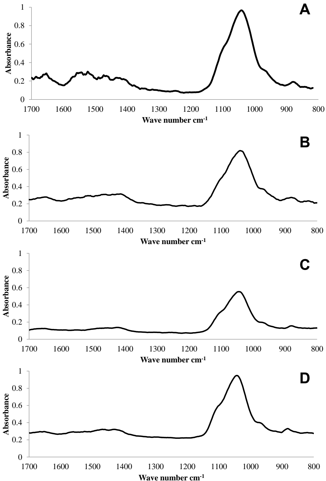
Figure 2: FTIR spectra (1700 - 800 \text{cm}^{-1} ) of dried powdered human dentine samples (n=5) that were A) untreated (control) or exposed to solutions of B) calcium hydroxide, C) white MTA or D) grey MTA over a 14-day period during dECM components extraction.
