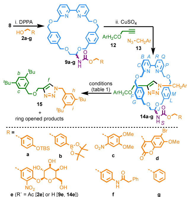
Scheme 2. Synthesis of macrocycles 9 , their conversion to rotaxanes 14 and their subsequent axle-releasing reactions ( Ar = 3,5\text{-di-}^t\text{Bu-C}_6\text{H}_3 ). Reagents and conditions: i. 2 , DPPA, K_2CO_3 , CH_2Cl_2 , rt; [31] ii. CuSO_4 , sodium ascorbate, THF– H_2O (10:1), rt, 16 h. [32]
