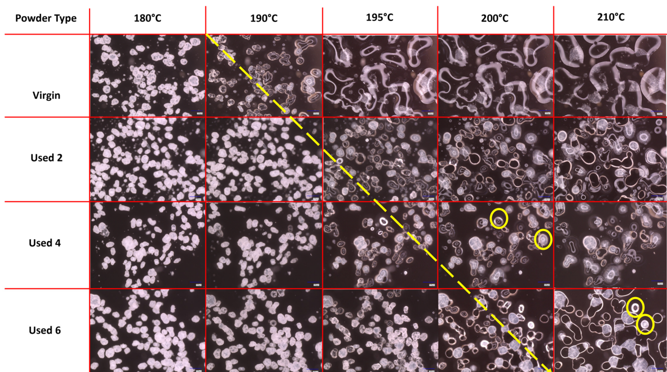
Figure 1. Powder melting and coalescence behaviour of virgin and used powder, observed using hot stage microscopy by heating samples at a constant heating rate of 10 °C/min. The theoretical yellow arrow indicates the change from particle softening to melting and coalescence during heating; yellow circles provide examples of incomplete melting and the presence of un-molten particle cores.
