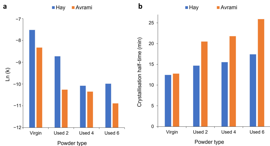
Figure 11. Comparison of the values of (a) k_p and (b) t_{1/2} using both the Hay and Avrami models, for each powder type, at an isothermal T_c of 165 ^{\circ}\text{C} .
