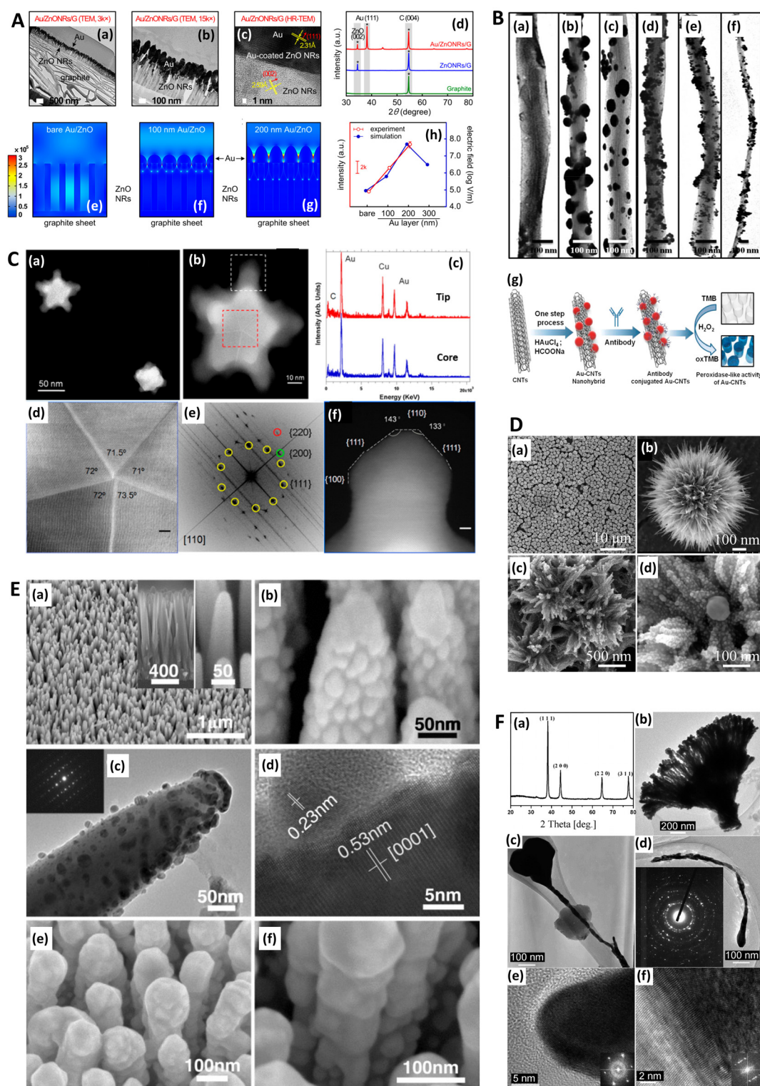
Fig. 2 Electron microscopies in SERS. A , Gold-coated zinc oxide nanorods (ZnO NRs) for SERS: experimental characterization and modeling. (a) and (b) Transmission electron microscopy (TEM) and (c) high-resolution transmission electron microscopy (HR-TEM) images of Au/ZnO NRs/G and (d) X-ray diffraction patterns of graphite, ZnO NRs/G, and Au/ZnO NRs/G. (e)–(g) Computational results of FEM models approximated from (e) bare Au as well as (f) 100 nm thick and (g) 200 nm thick Au layers coated onto ZnO NRs with heights of 400 nm on graphite sheets. (h) Similarity of experimental findings (Raman intensity) and FEM computational findings (maximum electric field) with three models. G = graphite. FEM = finite element method. Reprinted with permission from Kim (2017) © American Chemical Society. 128 B , TEM images of Au–CNT nanohybrids. (a) Carbon nanotubes (CNTs); (b) Au–CNT nanohybrids with ~60 nm-sized AuNPs; (c) Au–CNT nanohybrids with ~40 nm-sized Au NPs; (d) Au–CNT nanohybrids with
