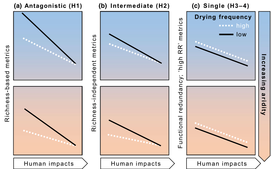
FIGURE 1 Hypothesized responses of invertebrate-based metrics to human impacts at river sites with high and low drying frequencies across a climatic gradient. Hypotheses (H) 1–4 are described in the text; (a) antagonistic, (b) intermediate and (c) single responses are sensu Côté et al. (2016)
