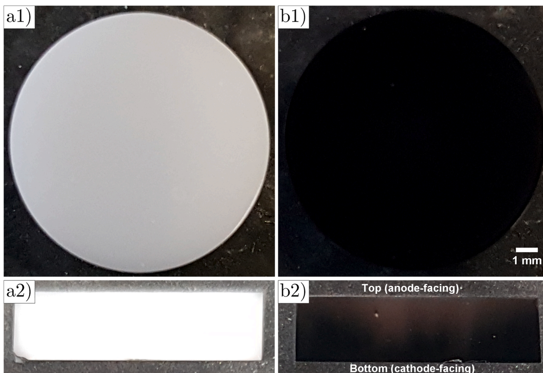
Fig. 2. Camera images of (a) untreated and (b) plasma treated zirconia from the bottom surface (labelled 1) and cross-sectional (labelled 2) views are shown. The bottom surface images (a1 and b1) clearly illustrate the complete transformation of zirconia from white to black after plasma treatment. The cross-sectional views reveal an internal colour gradient, with the bottom surface facing the cathode appearing darker and the top surface facing the anode appearing lighter.
