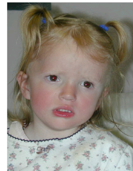
Individual 9 p.(Thr208Met)
