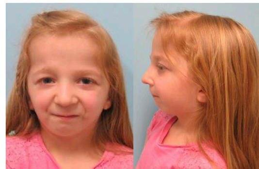
Individual 11 p.(Lys245Arg)
