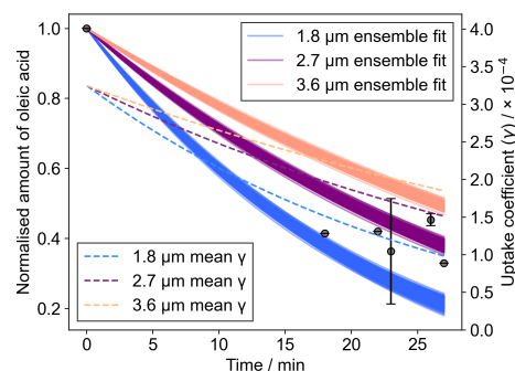
Figure 4. The decay of oleic acid followed experimentally using the area of the C = C Raman band at \sim 1650 \text{cm}^{-1} normalised to the \text{CH}_2 band at \sim 1452 \text{cm}^{-1} . Ensemble outputs from a pre-optimised model of oleic acid ozonolysis (Berkemeier et al., 2021) are presented for a range of initial film thicknesses in the range measured by WLI. The mean uptake coefficient ( \gamma ) for each ensemble, derived from the model output, is also plotted.
