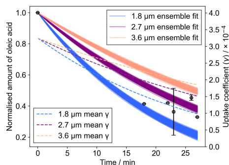
Figure 4. The decay of oleic acid followed experimentally using the area of the C = C Raman band at \sim 1650 \text{cm}^{-1} normalised to the \text{CH}_2 band at \sim 1452 \text{cm}^{-1} . Ensemble outputs from a pre-optimised model of oleic acid ozonolysis (Berkemeier et al., 2021) are presented for a range of initial film thicknesses in the range measured by WLI. The mean uptake coefficient ( \gamma ) for each ensemble, derived from the model output, is also plotted.
