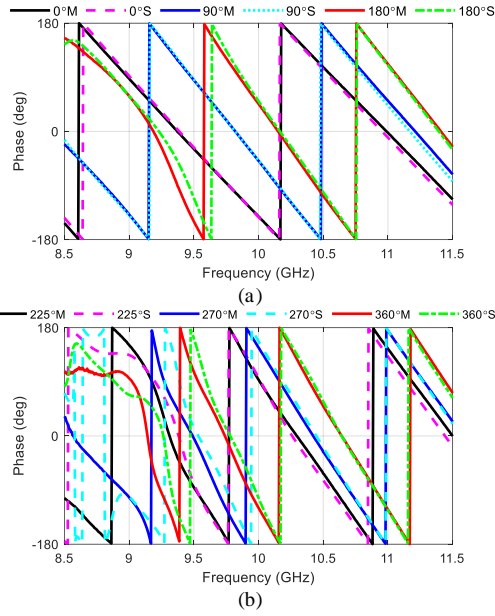
Fig. 12. The Measured S_{21} of the proposed uniform LM phase shifter. (a) 0° to 180° and (b) 180° to 360°. [M: is for measurement results and S is for simulated results]
